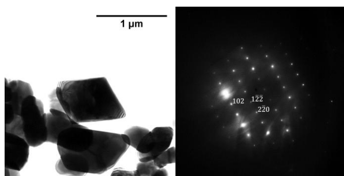
Fig. 6 TEM image of a hexagonal bipyramid crystal and power spectrum of image which serves to identify the crystal, zone axis [2\bar{2}\bar{1}]
