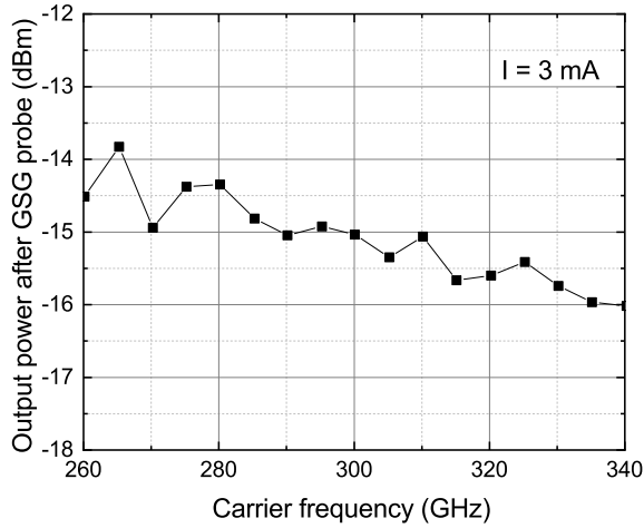
Fig. 2: Frequency evolution of generated power at UTC-PD output, connected to the GSG probe. The power level is measured at waveguide output, for 3 mA photo current inside the UTC-PD. The photodiode bias is -1 V.
