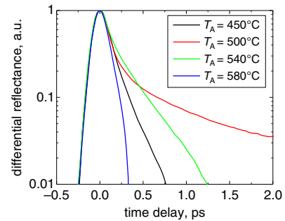
Fig. 2 Time-resolved photoreflectance measurements obtained on the LT-GaAs layers grown at 250^\circ\text{C} and annealed at T_A = 450, 500, 540 and 580^\circ\text{C}
