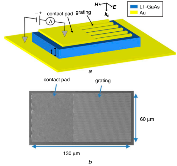
Fig. 1 Optical cavity LT-GaAs photoconductor
