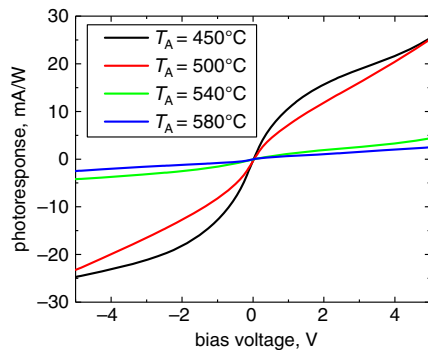
Fig. 4 Photoresponse-bias voltage characteristics measured on optical cavity photoconductors fabricated using LT-GaAs layers grown at 250^\circ\text{C} and annealed at T_A = 450, 500, 540 and 580^\circ\text{C}
