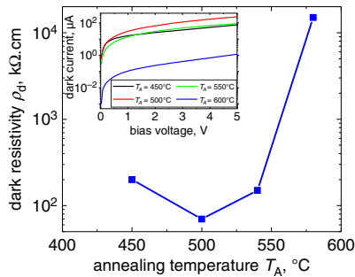
Fig. 3 Dark resistivity dependence on post-growth annealing temperature T_A . Inset: Dark current versus bias voltage obtained on the 60 \times 130 \mu\text{m}^2 area test structures
