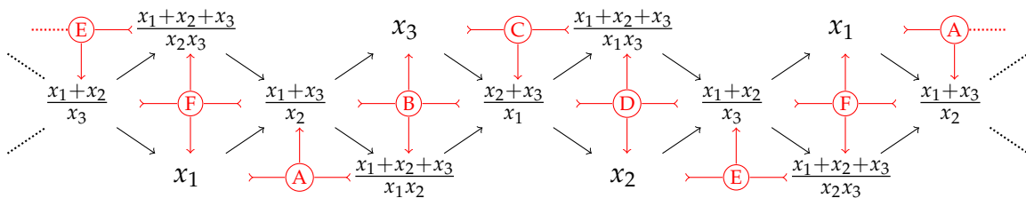
Figure 4: The facet-defining inequalities of the type cone \text{TC}(\mathcal{F}(B_\circ)) for the cluster fan of Figure 2 (right). See Theorem 16. The conventions are similar to Figure 3.
