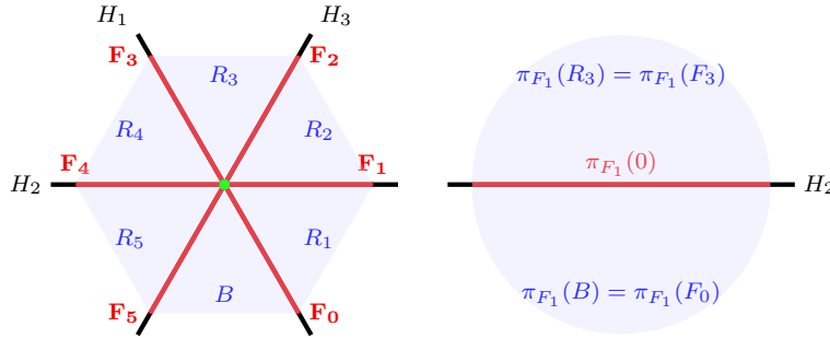
FIGURE 7. The map \pi_{F_1} from an arrangement \mathcal{A} to a subarrangement \mathcal{A}_{F_1} . See Example 4.5.
