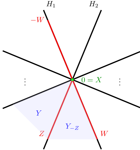
FIGURE 10. The construction of the join in the third case when X \subseteq Z \subseteq Y .
