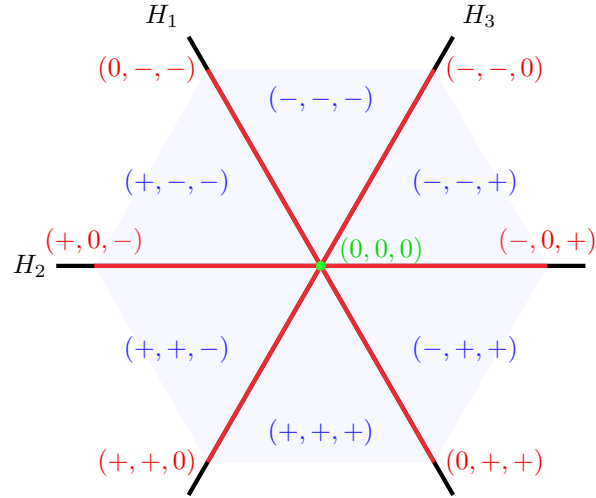
FIGURE 5. The type A_2 Coxeter arrangement where the faces are identified by their associated covectors. See Example 3.1.
