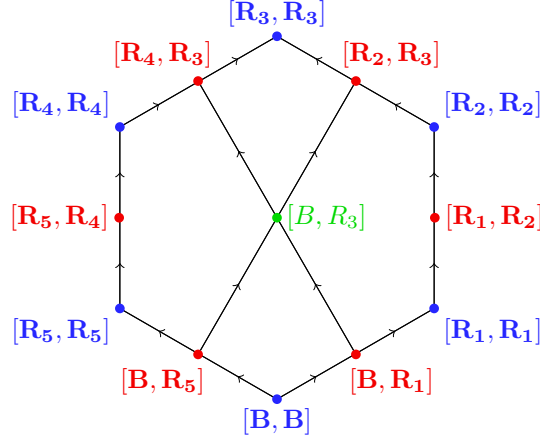
FIGURE 4. The facial weak order labeled by facial intervals for the type A_2 Coxeter arrangement. See Example 2.10.
