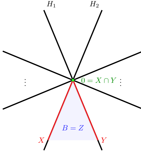
FIGURE 8. The construction of the join for the first case when X \cup Y \subseteq Z .
