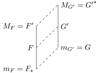
FIGURE 12. Meet-semidistributivity in the facial weak order.
