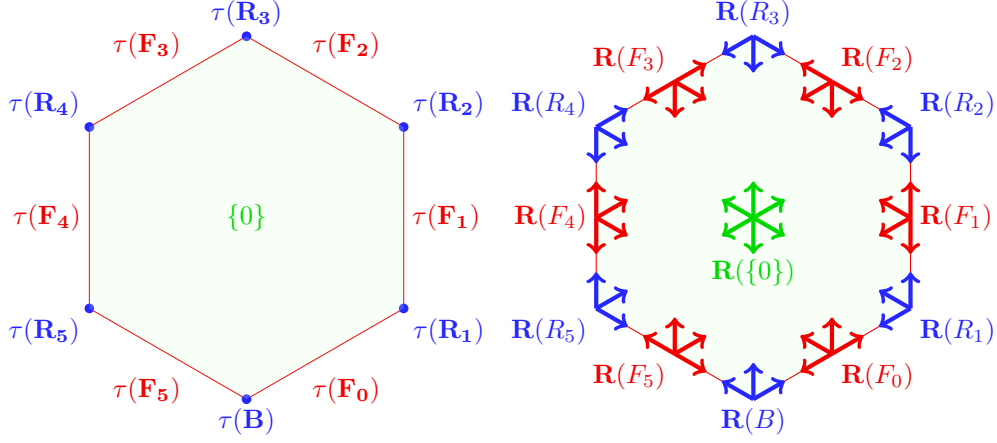
FIGURE 6. The type A_2 Coxeter arrangement. On the left is the zonotope created by the \tau map in Lemma 3.21. On the right we label each face with the root inversion set for that face. See Example 3.20 and Example 3.23.
