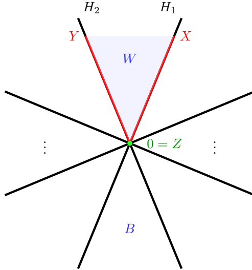
FIGURE 9. The construction of the join for the second case when Z \subseteq X \cap Y .
