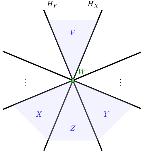
FIGURE 11. The construction of the join when X and Y are regions.
