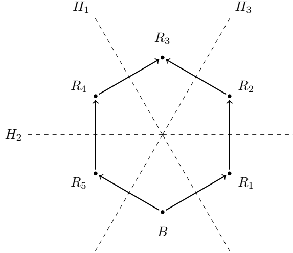
FIGURE 3. The lattice of regions associated to the type A_2 Coxeter arrangement. See Example 2.4.
