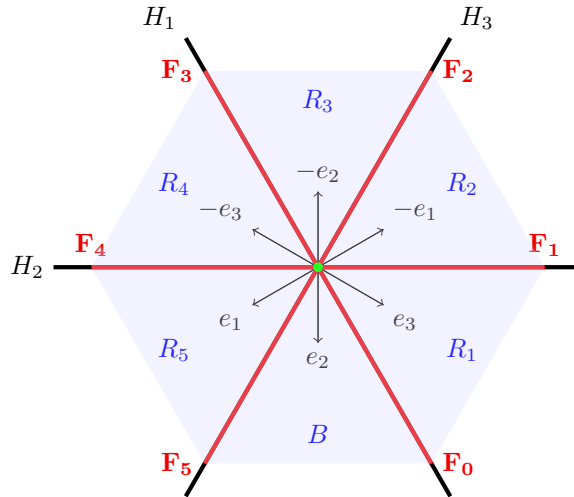
FIGURE 2. The type A_2 Coxeter arrangement where B is the intersection of the positive half-spaces of all hyperplanes. See Example 2.1.
