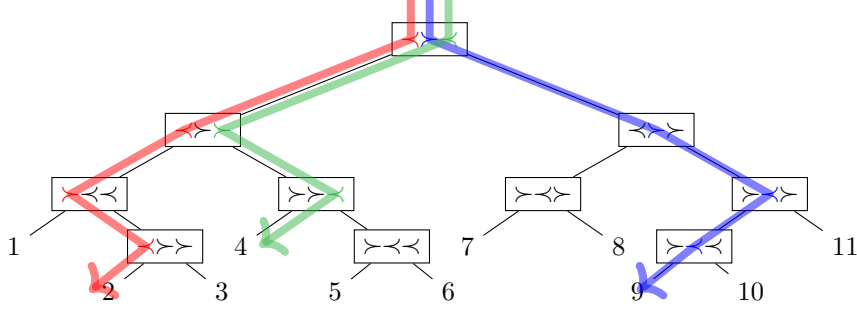
FIGURE 6. Traversing the syntax tree in parallel. The parallel routes are marked, and the parallel destination vector is \langle 2, 9, 4 \rangle_{11} .
