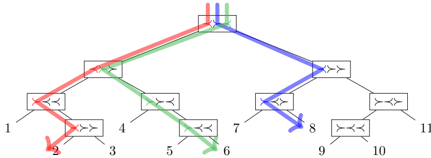
FIGURE 7. Traversing the syntax tree in series. The series routes are marked, and the series destination vector is \langle 2, 8, 6 \rangle_{11} .
