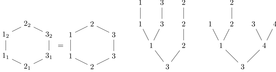
FIGURE 3. A 2-poset of degree 3 (left), a 3-poset of degree 3 (middle), and a 2-poset of degree 4 (right). See Definition 2.50.
