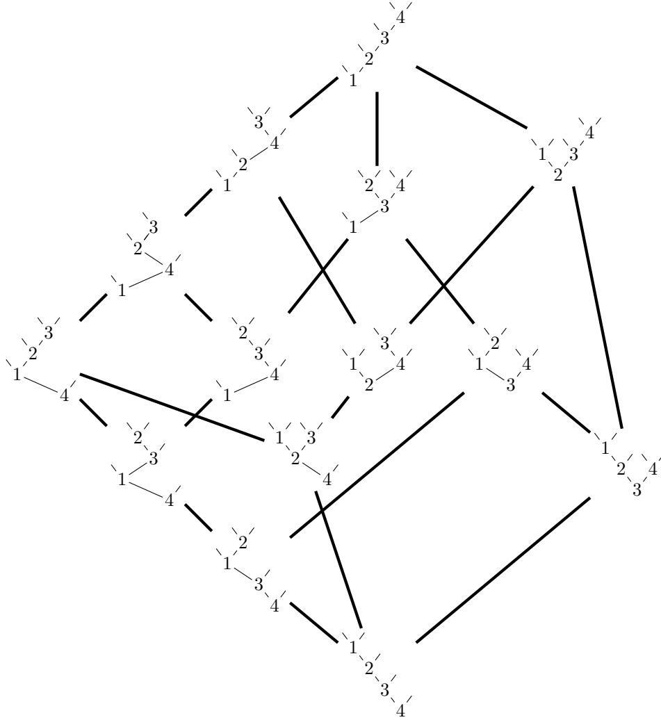
FIGURE 1. The Tamari lattice on binary trees. See Definition 2.33.
