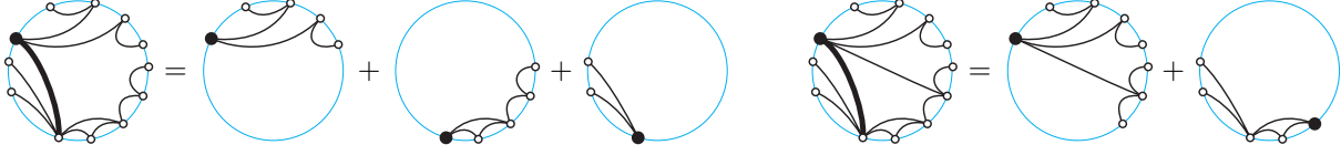
FIGURE 8. Decomposition of two rooted non-crossing connected arc diagrams, whose root and leftmost arc \alpha incident to the root are bolded. We obtain three subdiagrams when \alpha is an isthme (left), and two subdiagrams when \alpha is not an isthme (right). See Remark 4.25.
