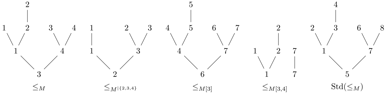
FIGURE 4. Shifts and standardization of multiposets. See Definitions 2.51 to 2.54.
