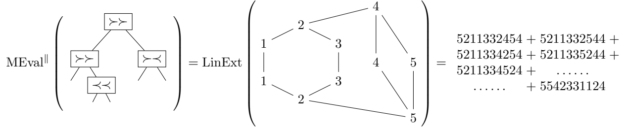
FIGURE 12. Illustration of Lemma 5.54.
