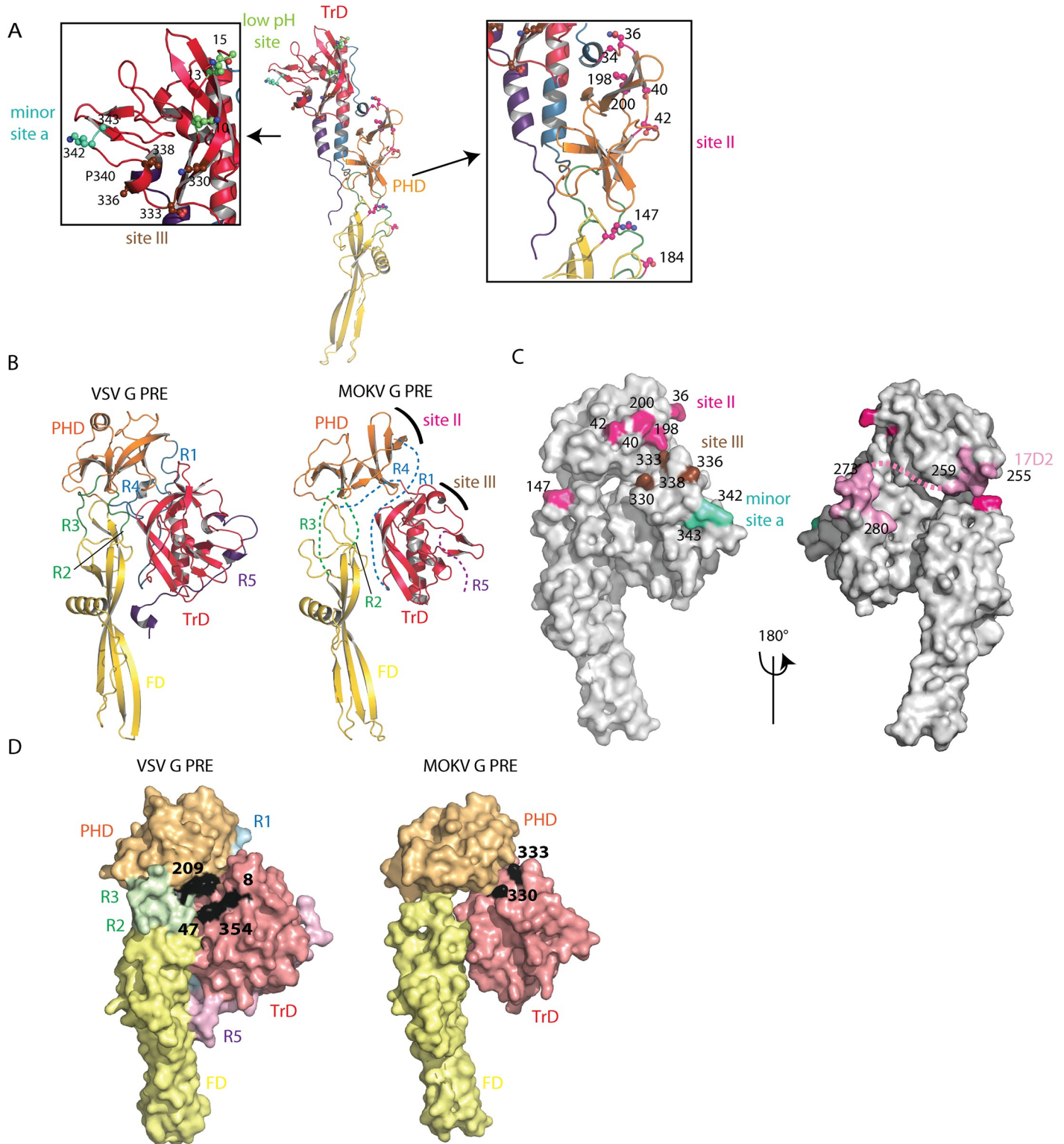
Fig 6. Antigenic sites or RABV positioned on MOKV G structure. A) Location of major antigenic sites II and III, minor antigenic site a, and low pH antigenic site. Residues that are found substituted in mutants escaping neutralization by MABs are indicated by their number and represented in ball and sticks form. They are colored in magenta for site II, in brown for site III, in cyan for minor site a, and in green for low pH antigenic site. Proline 340, which separates site III and minor site a, is also indicated. B) Model of MOKV G pre-fusion generated by superimposing MOKV G PHD, TrD, and FD domains on the corresponding domains of VSV G. The location of major antigenic sites II and III are indicated on the model. C) Surface representation of the modeled MOKV G pre-fusion state. Residues that are
