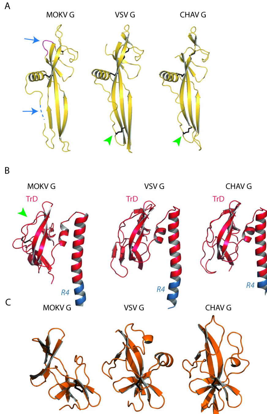
Fig 3. Comparison of the structure of MOKV G domains with those of VSV and CHAV G. A) Comparison of FDs of MOKV, VSV, and CHAV G. Blue arrows indicate additional segments present in all lyssaviruses G. The dotted line represents the missing segment in MOKV G structure. Green arrowheads indicate the disulfide bridge present in vesiculoviruses G but not in lyssaviruses G. B) Comparison of TrDs and R4 segment of MOKV, VSV, and CHAV G. Note that MOKV G helix is bent, whereas it is rather straight for CHAV G and VSV G. The green arrowhead indicates the extra disulfide bridge of lyssaviruses G. C) Comparison of PHDs of MOKV, VSV, and CHAV G.
