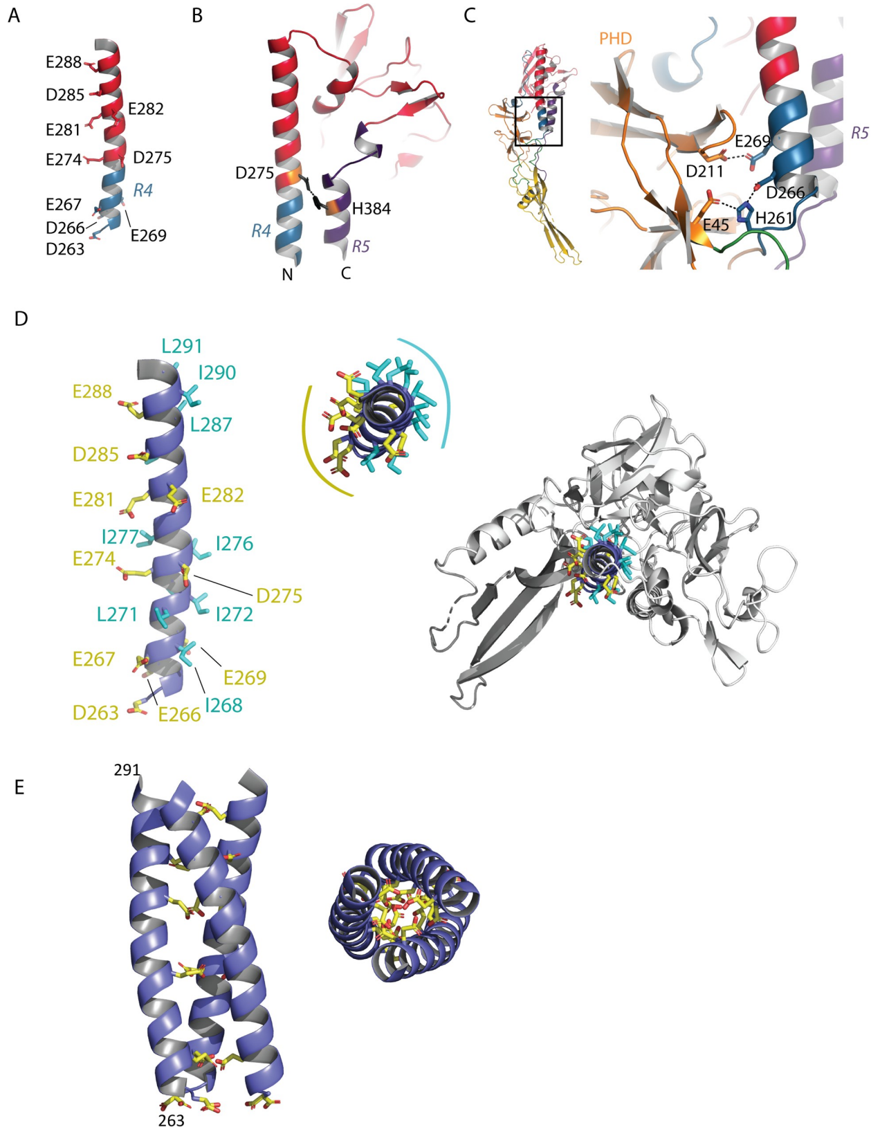
Fig 7. pH-sensitive molecular switches in MOKV G. A) Position of acidic residues on the TrD long helix. B) Lateral view of the TrD and segments R4 and R5 showing the interaction between D275 and H384 stabilizing the post-fusion state of MOKV G. C) Close up view on the pair of acidic residues (D211 in PHD and E269 in R4) facing each other in the post-fusion conformation of MOKV G and on the environment of H261 (in R4), which is sandwiched by D266 (in R4) and E45 (in PHD). D) View of the TrD long helix showing the disposition of hydrophobic (in cyan) and acidic (in yellow) residues. E) View of the TrD long helix showing the disposition of hydrophobic (in cyan) and acidic (in yellow) residues.
