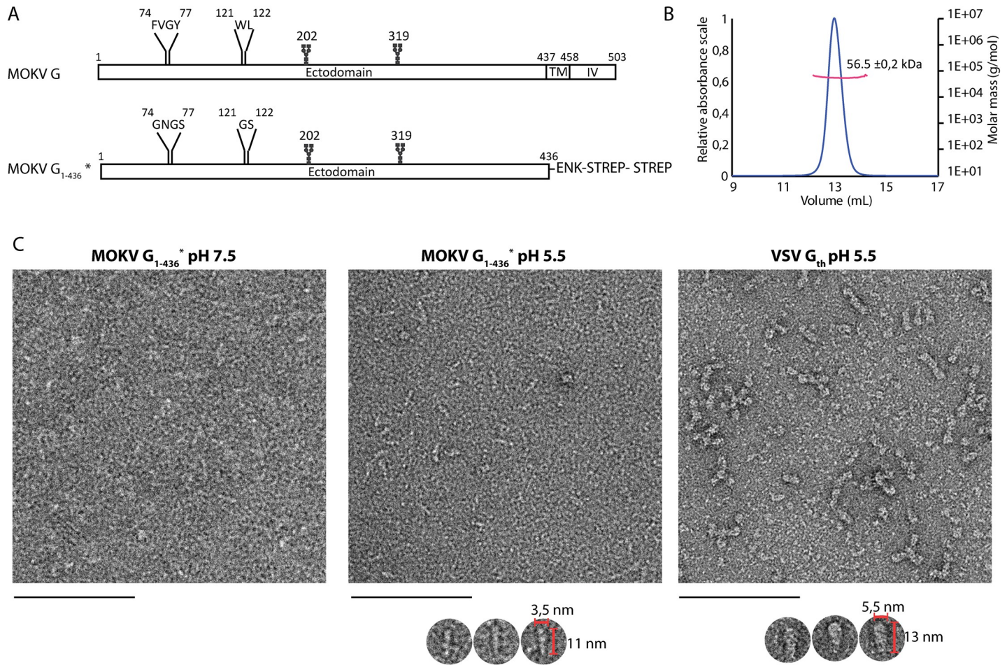
Fig 1. Construction, purification, and characterization of MOKV G 1-436 *. A) Bar diagram showing the organization of MOKV G and G 1-436 *. The N-glycosylation sites are indicated as well as the two fusion loops in G and the hydrophilic sequences that replace them in G 1-436 *. TM: transmembrane domain; IV: intraviral domain; ENK: enterokinase cleavage site; STREP: StrepTag. B) Molecular mass of MOKV G 1-436 * determined by SEC-MALS. C) Electron microscopy on negatively stained MOKV G 1-436 * at pH 7.5 and 5.5 and VSV G th at pH 5.5. At pH 7.5, no defined molecular shape of MOKV G 1-436 * can be identified. At pH 5.5, elongated structures can be distinguished as shown in the gallery below the micrograph. These structures are thinner than those observed with the post-fusion G th trimers. Scale bar: 100 nm.
