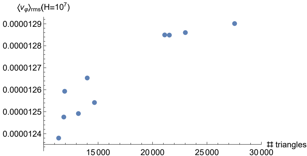
FIGURE 17. For H = 10^7 and \Delta T = 0.1 (giving \langle H \rangle \simeq 1.04 \times 10^7 ), and for v_\varphi = 0 on \partial\Omega , the root mean square of v_\varphi i.e. \|v_\varphi\|_{L^2} ((in Alfvén velocity v_A units)) obtained numerically is plotted as a function of the number of triangles of the mesh. The dispersion of the results on the left part is due to the fact that we do not use a single series of regular meshes.
