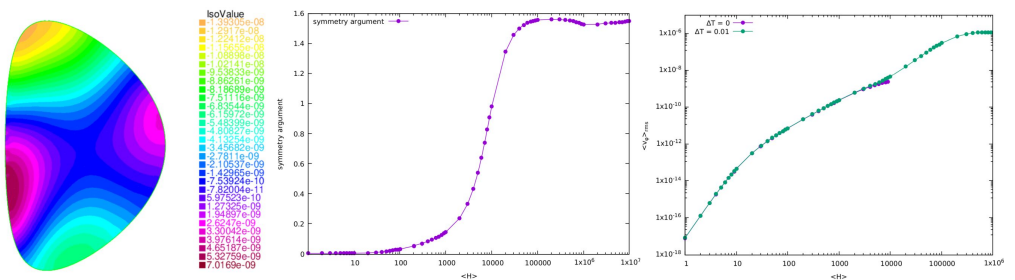
FIGURE 13. (left) Toroidal velocity v_\varphi field for H = 10^4 and \Delta T = 0.01 ; (middle) Symmetry argument \chi = \arctan(V_{\text{sym}}/V_{\text{anti}}) for \Delta T = 0.01 ; (right) \langle v_\varphi \rangle_{\text{rms}} for \Delta T equal to 0 and 0.01 as a function of \langle H \rangle .
