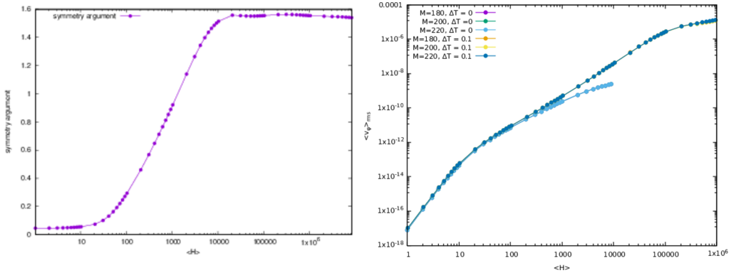
FIGURE 12. (left) Symmetry argument \chi = \arctan(V_{\text{sym}}/V_{\text{anti}}) for \Delta T = 0.1 ; (right) \langle v_\varphi \rangle_{\text{rms}} for \Delta T equal to 0 and 0.1 as a function of \langle H \rangle .
