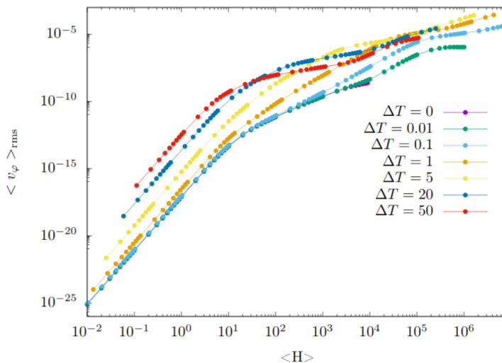
FIGURE 5. Root mean square of the toroidal velocity, \langle v_\varphi \rangle_{\text{rms}} , (in Alfvén velocity v_A units) as a function of \langle H \rangle for different values of \Delta T .
