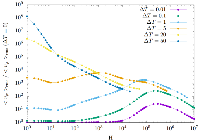
FIGURE 8. For the same data as in Figure 6, plots of the ratio \langle v_\varphi \rangle_{\text{rms}}(\Delta T \neq 0) / \langle v_\varphi \rangle_{\text{rms}}(\Delta T = 0) as a function of H (Hartmann number at the bottom of the tokamak) for different values of \Delta T .
