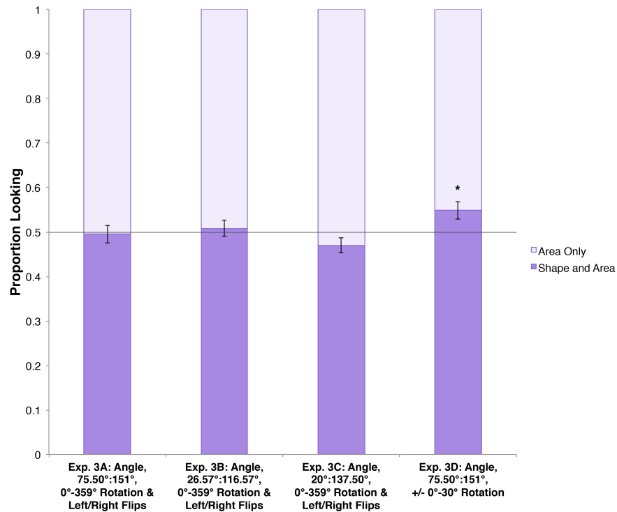
Figure 7. Proportion of looking to angle changes in Experiments 3A-3D. Infants did not detect angle changes in the figures varying by a 2-or-more-fold difference in angle when figures presented unlimited variations in orientation and sense (Experiments 3A-3C), but infants did detect changes in figures varying by a 2-fold difference in angle when figures presented limited variations in orientation and no changes in sense (Experiment 3D). The gray line at 0.5 indicates equal looking. * p < .05 , two-tailed.
