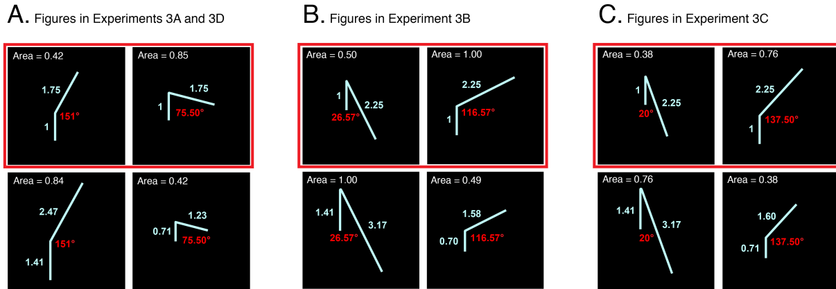
Figure 6. A. Context figures, angle-and-area change figures, and area-only change figures for Experiments 3A and 3D, B. 3B, and C. 3C. The figures bounded by red boxes are different angles and different areas, and they were presented in alternation on one side of the screen. On the other side of the screen, an area change but no angle change was presented. Half of the infants saw the left figure in each red box alternate with the larger version of itself depicted directly below it, and half of the infants saw the right figure in each red box alternate with the smaller version of itself, depicted directly below it. The length, angle, and area measurements are provided for each figure and are normalized for each condition.
