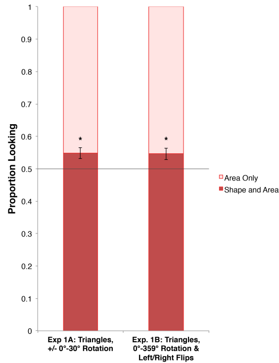
Figure 3. Proportion of looking to shape changes in Experiments 1A and 1B. Infants detected shape changes in connected triangles over limited (Experiment 1A) and unlimited variations in orientation and sense (Experiment 1B). The gray line at 0.5 indicates equal looking. * p < .05 , two-tailed.
