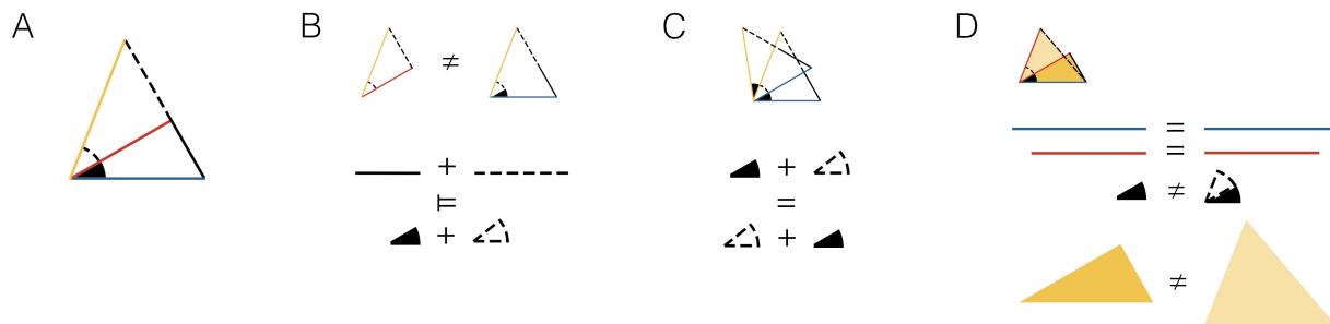
Figure 1. A. The smaller triangle with red, blue, and black sides sits inside the larger triangle with yellow, blue, and black sides. B. When the black side of the smaller triangle is extended to make the larger triangle, then the opposite angle size gets larger as well. C. Only when figures are presented at different orientations are individual line orientations dissociated from angle sizes. D. The area of a triangle changes as one angle varies if the adjacent side lengths are held constant.
