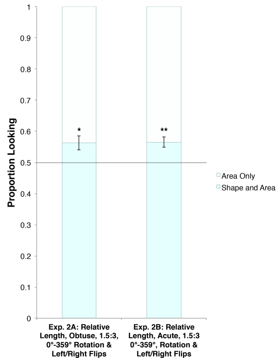
Figure 5. Proportion of looking to relative length changes in Experiments 2A and 2B. Infants detected relative length changes in open obtuse (Experiment 2A) and acute (Experiment 2B) figures over unlimited variations in orientation and sense. The gray line at 0.5 indicates equal looking. * p < .05 , ** p < .01 , two-tailed.
