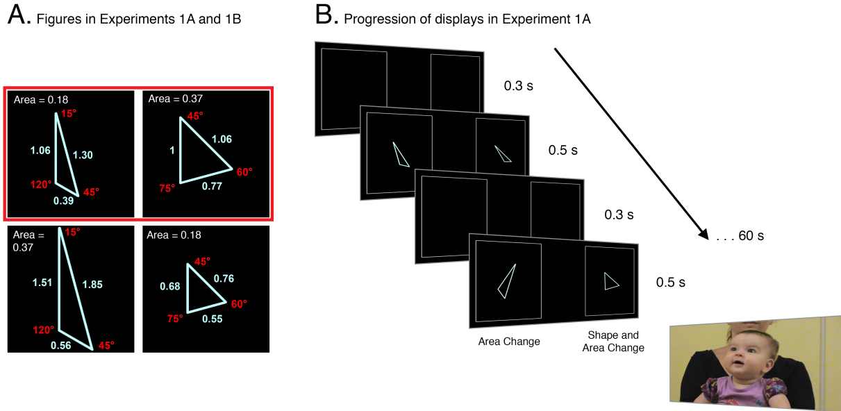
Figure 2. A. Context figures, shape-and-area change figures, and area-only change figures for Experiments 1A and 1B. The figures bounded by red boxes are different shapes and different sizes, and they were presented in alternation on one side of the screen. On the other side of the screen, a size change but no shape change was presented. Half of the infants saw the left figure in the red box alternate with the larger version of itself depicted directly below it, and half of the infants saw the right figure in the red box alternate with the smaller version of itself, depicted directly below it. The length, angle, and area measurements are provided for each figure. B. Progression of displays in Experiment 1A. On one side of the screen, infants saw a triangle changing in shape and in area by a factor of 2, and on the other side of the screen infants saw a triangle changing in area only (also by a factor of 2). At each presentation, the figures varied randomly in position, size, and orientation ( \pm 0^\circ - 30^\circ ). The type of change switched sides between trials, and the starting location of the shape-and-area change side was counterbalanced across infants.
