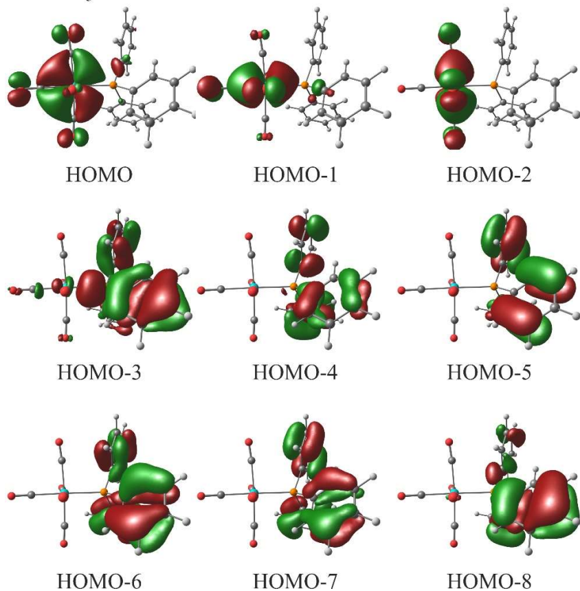
Figure 5. Kohn-Sham orbitals of Ph_3PMo(CO)_5 obtained at the LC- \omega PBEh/Def2-TZVP level of theory. Isosurface value: 0.03 a.u.
