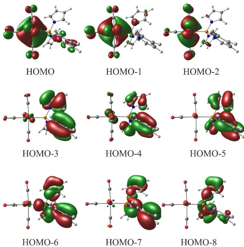
Figure 8. Kohn-Sham orbitals of Pyrl_3PMo(CO)_5 obtained at the LC- \omega PBEh/Def2-TZVP level of theory. Isosurface value: 0.03 a.u.
