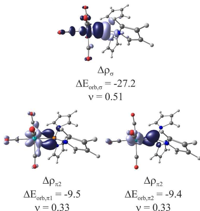
Figure 9. Contours of deformation density \Delta\rho_{\sigma/\pi} connected with the pairs of interacting orbitals in the PPyrl 3 P-Mo(CO) 5 complex. Light purple surfaces represent a loss of electron density and dark blue surfaces, a gain of electron density. The associated orbital interaction energies \Delta E_{\text{orb}} are given in kcal/mol. \nu is the eigenvalue indicating the size of the charge flow. Isosurface value: 0.0025 a.u.
