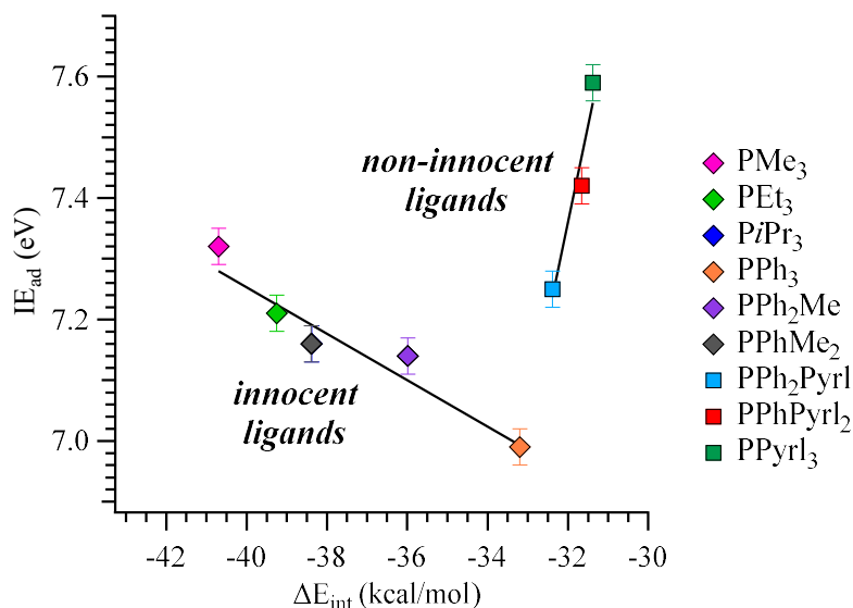
Figure 10. Correlation plots between \text{IE}_{\text{ad}} and \Delta E_{\text{int}} (values given in Tables 1 and 2) for all ligands studied. Note that the points for L = \text{P}i\text{Pr}_3 and L = \text{PPhMe}_2 are superimposed.
