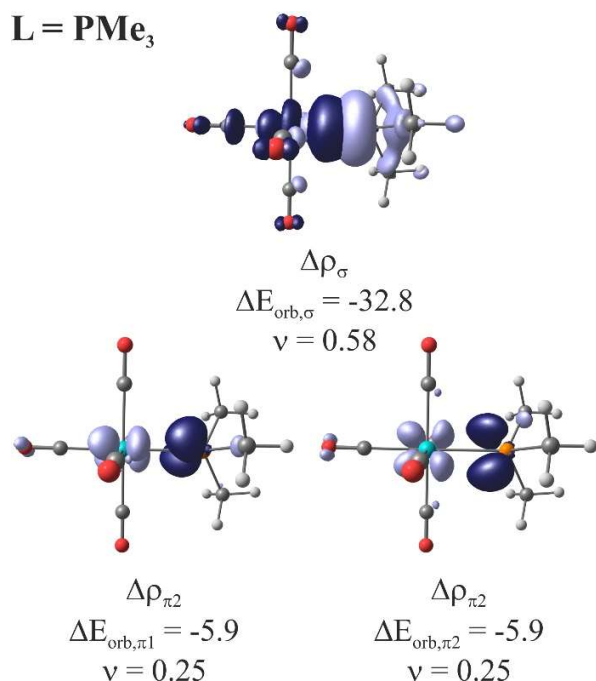
Figure 4. Contours of deformation density \Delta\rho_{\sigma/\pi} connected with the pairs of interacting orbitals in the \text{Me}_3\text{P-Mo}(\text{CO})_5 complex. Light purple surfaces represent a loss of electron density and dark blue surfaces, a gain of electron density. The associated orbital interaction energies \Delta E_{\text{orb}} are given in kcal/mol. \nu is the eigenvalue indicating the size of the charge flow. Isosurface value: 0.0025 a.u.
