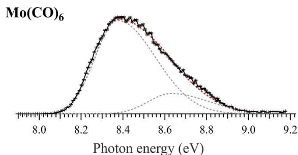
Figure 1. SPES of the Mo(CO) 6 + ion recorded in the 7.9-9.2 eV energy range. Plain lines represent the experimental spectrum whereas dotted lines are the asymmetric Gaussian curves used to fit the data.
