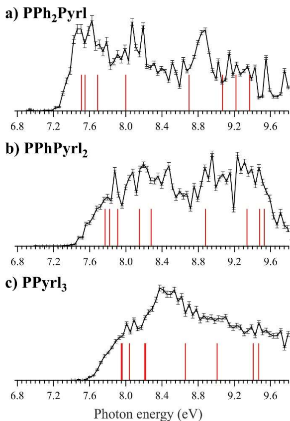
Figure 7. SPES of the \text{LMo(CO)}_5^{+} ions for the \text{PPh}_x\text{Pyr}_{1(3-x)} series recorded in the 6.8-9.7 eV energy range. Red lines represent the calculated energies of the first HOMOs of the neutral complexes.
