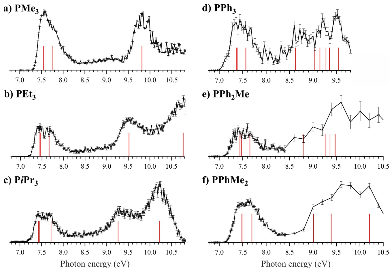
Figure 2. SPES of the \text{LMo}(\text{CO})_5^{+} ions for the a)-c) \text{L}=\text{PR}_3 (with \text{R} = \text{alkyl} ) and d)-f) \text{L}=\text{PPh}_x\text{Me}_{(3-x)} series recorded in the 6.8-10.5 eV energy range. Red sticks represent the calculated energies of the first HOMOs of the neutral complexes. Because of a lack of experiment time, the spectra e) and f) were recorded in two steps: a first one from 6.6 to 8.4 eV with 20 meV steps and a second one from 8.4 to 10.5 eV with 200 meV steps.
