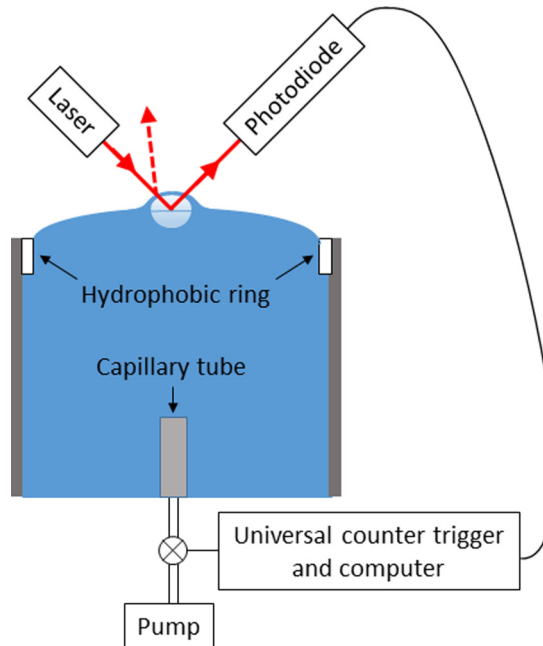
FIG. 1. Setup used to form bubbles and to measure their lifetimes on the surface of the liquid bath. The dashed red arrow corresponds to the reflection of the laser beam when a bubble is at the interface, while the solid red arrow corresponds to the reflection of the laser beam when there is no bubble at the interface.
