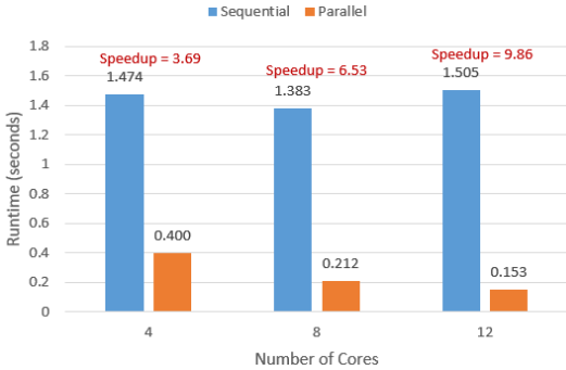
Fig. 11. The effect of increasing number of cores on runtime.
