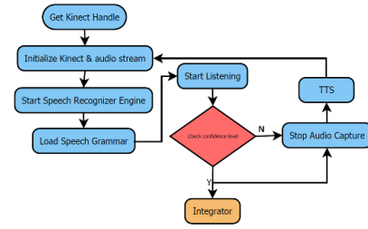
Fig. 3. We use the MSR speech recognition software on the detected audio stream.
