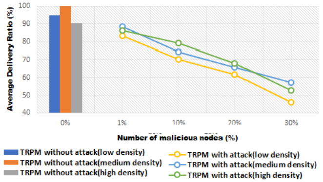
Fig. 7. Gray-hole attack: The average Packet Delivery Ratio vs number of Gray-hole attacker nodes
