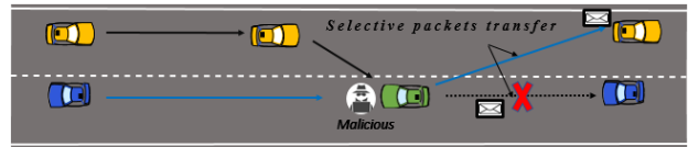
Fig. 3. Gray-hole attack principle.
