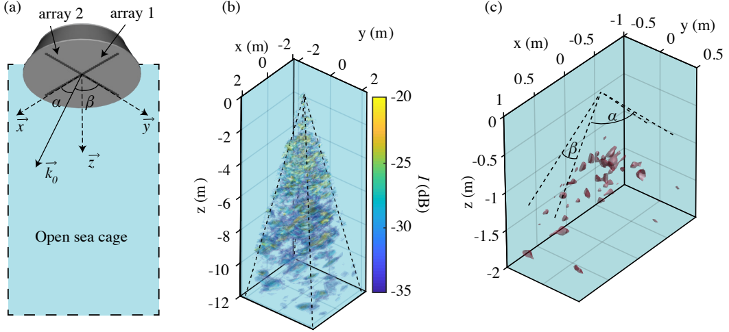
FIG. 1. (a) Scheme of the Seapix sonar probe positionned at the surface of the open sea cage. (b) Snapshot of a volumetric scan of a cage (backscattered acoustic intensity I ). (c) Isosurface representation of the shallow scan ( z < 2 m). Hot spots represent the closed volumes for which TS > -31 dB.
