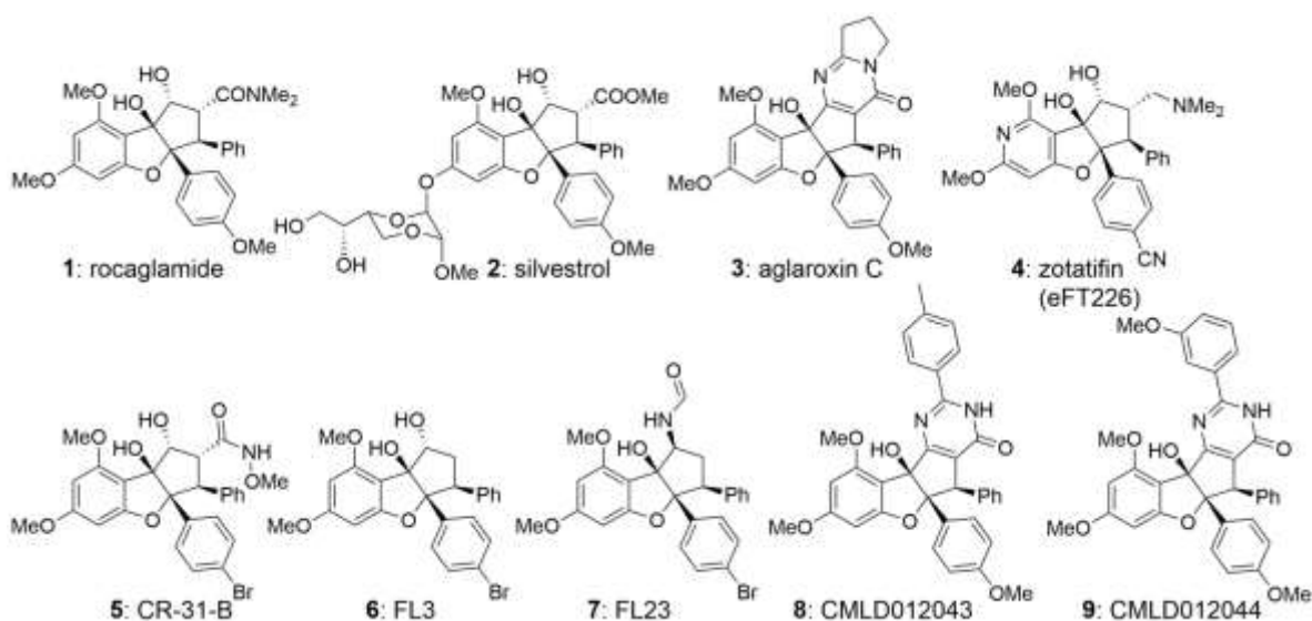
Figure 1. Natural (1-3) and synthetic (4-9) flavaglines with demonstrated antiviral activities.
