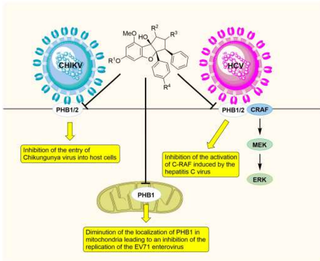
Figure 3. Antiviral effects of flavaglines mediated by PHBs.
