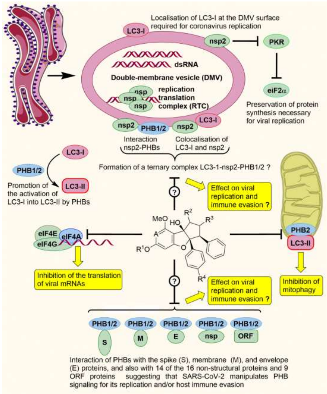
Figure 4. Putative effects of flavaglines on SARS-Cov2.
