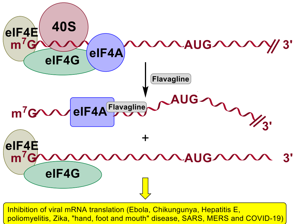
Figure 2. Structure and role in viral translation of the eIF4F complex. eIF4F includes the helicase eIF4A that unwinds the highly structured 5' untranslated region (5'-UTR) sequence of some viral RNAs, the cap-binding protein eIF4E, and the scaffold protein eIF4G. Flavaglines stabilize the interaction between eIF4A and the 5'UTR by altering the conformation of both eIF4A and the mRNA. As a consequence, eIF4A recycling is blocked, which leads to an inhibition of cap-dependent translation. AUG, translation initiation codon. 40S, small ribosome subunit, m 7 G, 7-methylguanosine located at the 5' end of the mRNA to which eIF4E binds.
