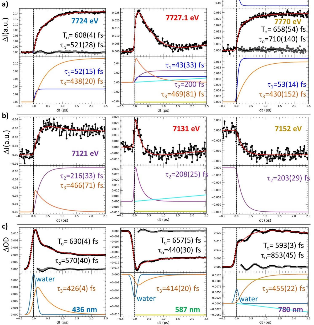
Fig. 8 Independent fit. Independent fits of the time traces of XANES at the Co (a) and Fe (b) edges and OD (c), resolving different components \tau_i to the signals. The residual between the signal and fits with exponential laws evidence damped oscillations of OD and some XANES data with period T_o and damping timescale \tau_o . For OD data the water response, exhibiting Gaussian response, was measured independently and included in the fit.
