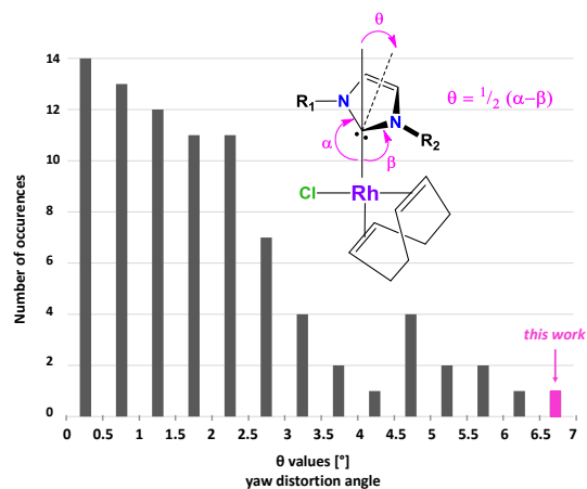
Figure 3. Distribution of yaw distortion angle values in structurally characterized \text{Rh}(\text{NHC})(\text{COD})\text{Cl} complexes. Analysis performed on 85 independent crystal structures. When several complexes are found in the asymmetric unit, the average \theta value is considered.
