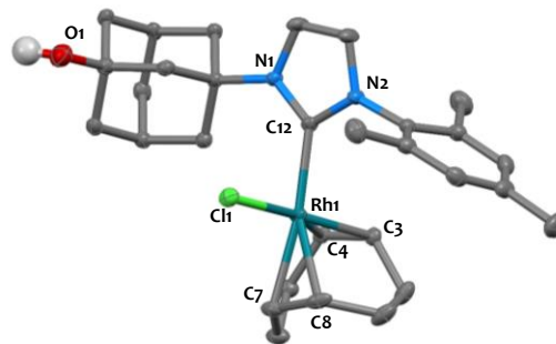
Figure 2. Solid-state molecular structure of 3 (30% probability ellipsoids). Hydrogen atoms, except that of the hydroxyl group have been omitted for clarity. Selected bond distances (Å) and angles (°): Rh1-Cl1 = 2.381(1); Rh1-C12 = 2.068(5); Rh1-C3 = 2.114(5); Rh1-C4 = 2.106(5); Rh1-C7 = 2.180(5); Rh1-C8 = 2.153(5); N1-C12 = 1.366(6); N2-C12 = 1.358(6); N1-C12-N2 = 103.9(4); C12-Rh1-Cl1 = 87.5(1); Rh1-C12-N1 = 134.2(4); Rh1-C12-N2 = 120.7(3).
