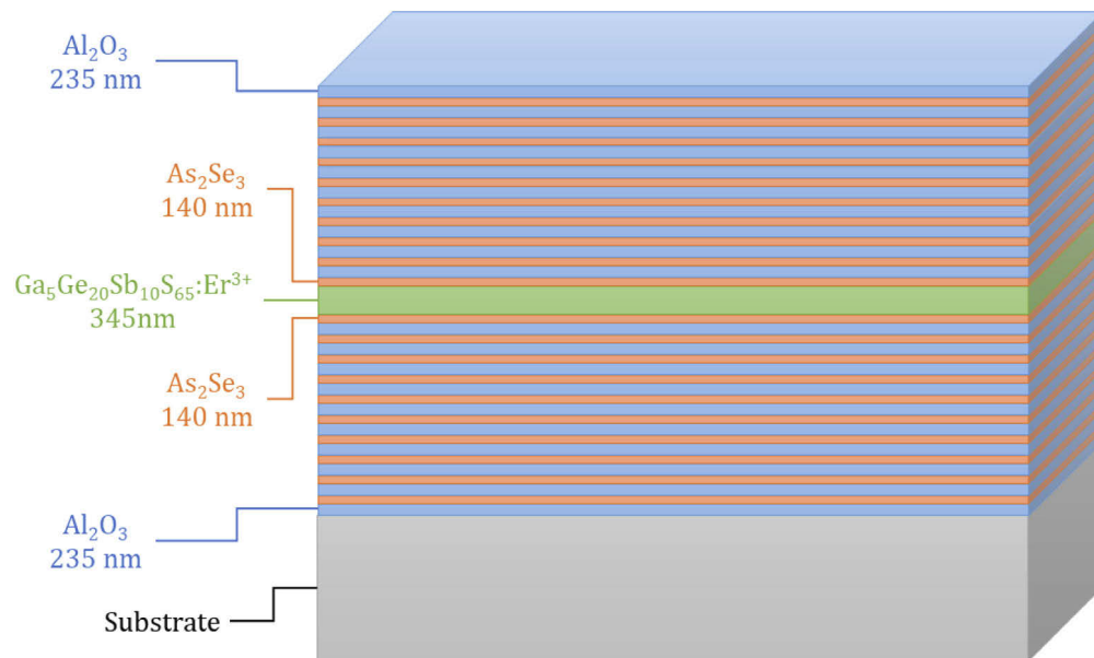
Fig. 6. Schematic representation of the Ga 5 Ge 20 Sb 10 S 65 :Er 3+ optical cavity enclosed between two 20-layer Al 2 O 3 -As 2 Se 3 BRs.
