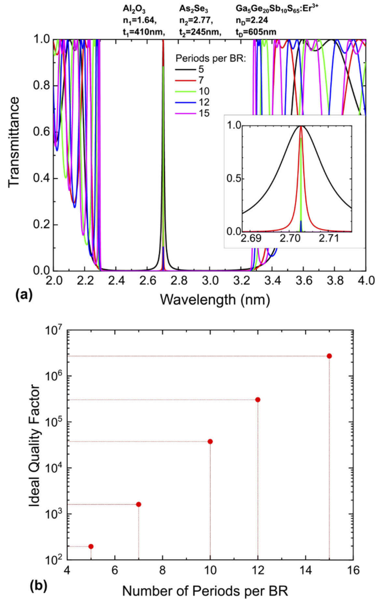
Fig. 10. (a) Transmission spectra of vertical cavities calculated via the transfer matrix formalism for operation within the {}^4I_{11/2} \rightarrow {}^4I_{13/2} \text{Er}^{3+} emission band, showing the effect of different number of BR periods on the stop-band profile; (b) estimate of the ideal cavity quality factor as a function of the number of iterations of the BR layer pairs. This represents an ideal case in which absorption is zero, so actual cavity quality factors are expected to be sensibly lower.
