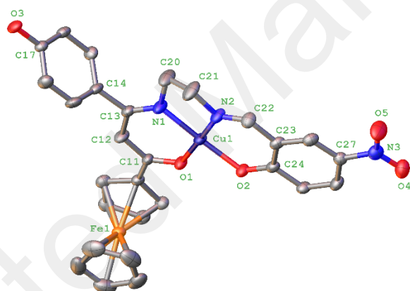
Figure 2. Molecular structure of complex 3 (molecule A ) with numbering scheme for selected atoms. Hydrogen atoms are omitted for clarity. Thermal ellipsoids are drawn at 50 % probability level.
