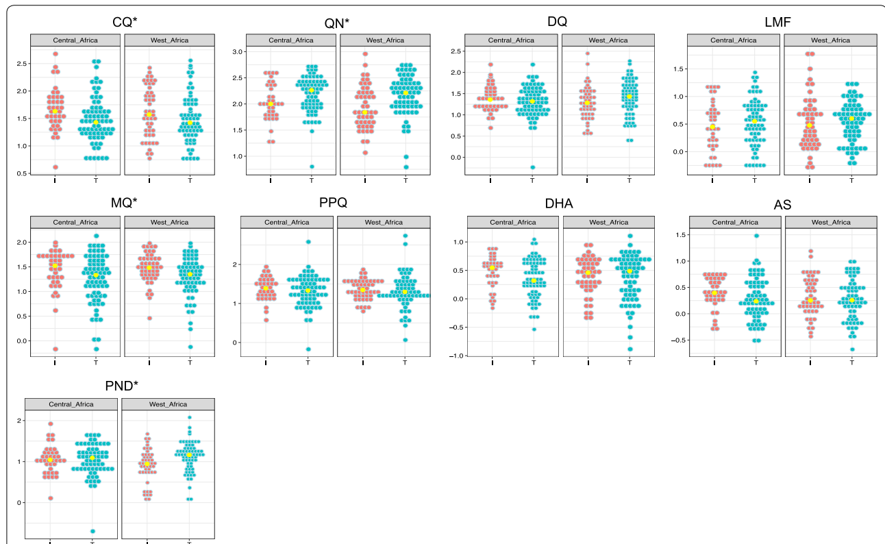
Fig. 1 Dot plot of the IC 50 values distribution of P. falciparum isolates from West Africa and Central Africa for chloroquine (CQ), quinine (QN), desethylamodiaquine (DQ), lumefantrine (LMF), mefloquine (MQ), piperiaquine (PPQ), dihydroartemisinin (DHA), artesunate (AS) and pyronaridine (PND) according to I356T. Each dot represents the log 10 (IC 50 ) for each isolate, red dots represent wild type I356 isolates (I), blue dots mutant 356T isolates (T) and yellow dots the log 10 (median IC 50 ) value for each drug. The y-axis represents the log 10 (IC 50 ) in nM. * Significant differences were found between wild type (I356) and mutant (356T) in West Africa (QN: p = 0.001, MQ: p = 0.01, PND: p = 0.005) and in Central Africa (QN: p = 0.02, MQ: p = 0.04, CQ: p = 0.01)
