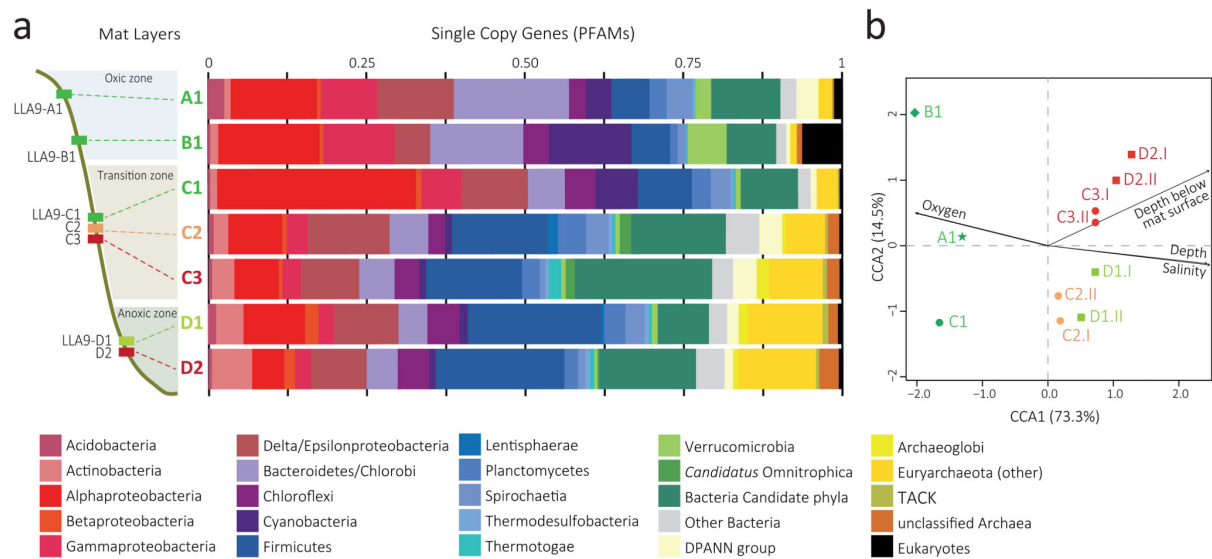
Fig. 1. Microbial diversity in microbial mat metagenomes along a redox gradient in a pond from the Salar de Llamara (Atacama Desert, Chile). (a) Overall community composition of metagenomic assemblies inferred from the phylogenetic assignment of PFAMs corresponding to 237 single copy genes. Layers LLA9-C2, C3, D1 and D2 correspond to merged metagenomes (see Supplementary Fig. 4a for individual replicates). Relatively abundant Candidatus Omnithrophica and Archaeoglobi are highlighted independently from their respective bacterial and archaeal clades. Detailed classification of archaea and bacterial candidate divisions is shown in Supplementary Fig. 4b-c. (b) Canonical correspondence analysis (CCA) plot based on normalized COG frequencies in individual metagenome datasets showing the similarity between replicate metagenomes and how the different metagenomes correlate with local environmental conditions (see also Supplementary Fig. 5).
