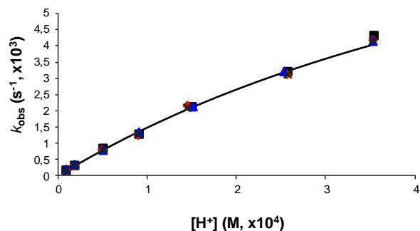
Figure 1. Dependence of the pseudo-first-order rate constants ( k obs ) on the concentration of H + and Cu(II) ions for the [Mn(PC2A-BP)] complex. The excess of the exchanging metal ion was ×10(■), ×20(●), ×30(▲) and ×40(×) folds. The line corresponds to the best fit of the k obs values to eqn. 2.
