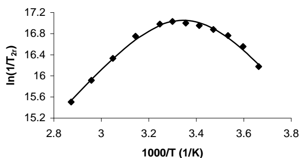
Figure 2. Temperature dependence of the reduced ^{17}\text{O} transverse relaxation rates for [Mn(PC2A-BP)] at 9.4 T and pH 7.4. The line corresponds to the best fit of the data.
