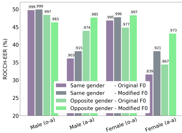
Figure 2: EER (%) score obtained by the ASV evaluation system on Librispeech tests sets. The C_{lr}^{min} score is displayed on the top of each bar. Multiple pipelines setups are reported for the gender selection and F0 modification. o – original, a – anonymized speech data for enrollment and trial parts. Entry “Same gender - Original F0” corresponds to the challenge baseline system.
