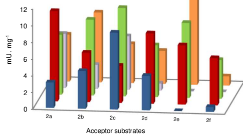
Chart 1. Specific activities of wild type, L382F, D470I, F435I, L191I TK_{gst} toward aliphatic aldehydes 2a-f as acceptors and HPA as donor. Enzyme reactions were carried out with 2a-f (100 mM), HPA (50 mM), purified enzyme (0.4 mg · mL -1 ), at pH 7.2 and 50 °C and incubated overnight.
