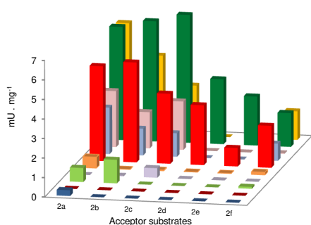
Chart 2. Specific activities of wild type, L382F, D470I, F435I, L191I, H102L/H474S, H102L/H474S/L382F, H102L/H474S/D470I, H102L/H474S/F435I, H102L/H474S/L191I toward aliphatic aldehydes 2a-f as acceptors and 2-oxobutyrate 1b as donor. Enzyme reactions were carried out with 2a-f (100 mM), 1b (50 mM), at, purified enzyme (0.4 mg · mL -1 ), at pH 7.2 and 50 °C and incubated overnight.
