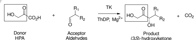
Scheme 1. Irreversible reaction catalyzed by TKs in the presence of hydroxypyruvate (HPA) as donor substrate with aldehydes as acceptor substrates.
