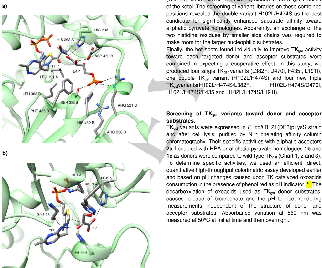
Figure 1. Model of wild-type TK gst based on the X-ray crystal structure of TK ban (PDB entry 3M49) with a) natural acceptor substrate D-erythrose-4-phosphate (E4P) and b) hydroxypyruvate (HPA) as donor. The model was built using Modeler 9.14 and Chimera.
