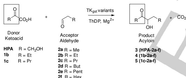
Scheme 2. Aliphatic acyloin synthesis catalyzed by TK gst variants in the presence of aliphatic pyruvate homologues as donors with aliphatic aldehydes as acceptors.
