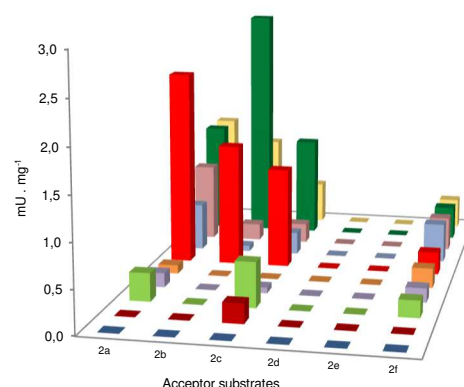
Chart 3. Specific activities of wild type, L382F, D470I, F435I, L191I, H102L/H474S, H102L/H474S/L382F, H102L/H474S/D470I, H102L/H474S/F435I, H102L/H474S/L191I toward aliphatic aldehydes 2a-f as acceptors and 2-oxovalerate 1c as donor. Enzyme reactions were carried out with 2a-f (100 mM), 1c (50 mM), at, purified enzyme (0.4 mg · mL -1 ), at pH 7.2 and at 50 °C and incubated overnight.
