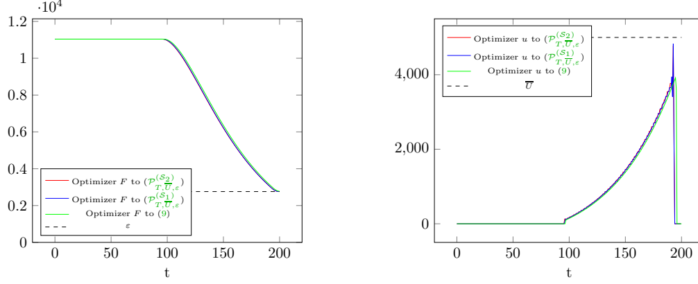
Figure 4: Solution of the optimal control problems (\mathcal{P}_{T, \bar{U}, \epsilon}^{(S_1)}) , (\mathcal{P}_{T, \bar{U}, \epsilon}^{(S_2)}) and (9) with T = 200 , \bar{U} = 5000 , \nu_E = 0.05 , and \epsilon = \bar{F}/4 .
