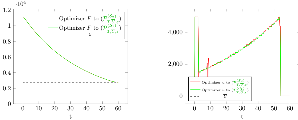
Figure 2: Solution of the optimal control problems (\mathcal{P}_{T,\bar{U},\varepsilon}^{(S_1)}) and (\mathcal{P}_{T,\bar{U},\varepsilon}^{(S_2)}) with T = 60 , \bar{U} = 5000 , \nu_E = 0.05 , and \varepsilon = \bar{F}/4 .
