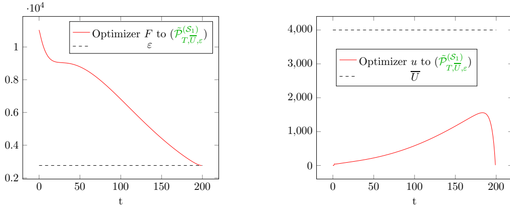
Figure 5: Solution of the optimal control problems (\tilde{\mathcal{P}}_{T, \bar{U}, \varepsilon}^{(\mathcal{S}_1)}) with T = 200 , \bar{U} = 4000 , \nu_E = 0.05 and \varepsilon = \bar{F}/4 .
