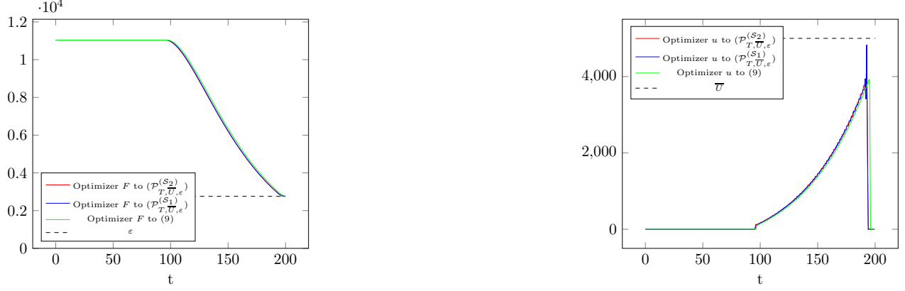
Figure 4: Solution of the optimal control problems (\mathcal{P}_{T,\bar{U},\varepsilon}^{(S_1)}) , (\mathcal{P}_{T,\bar{U},\varepsilon}^{(S_2)}) and (9) with T = 200 , \bar{U} = 5000 , \nu_E = 0.05 , and \varepsilon = \bar{F}/4 .
