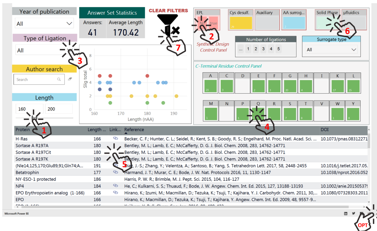
Figure 2. General control panel of the Protein Chemical Synthesis DataBase (PCS-db).
