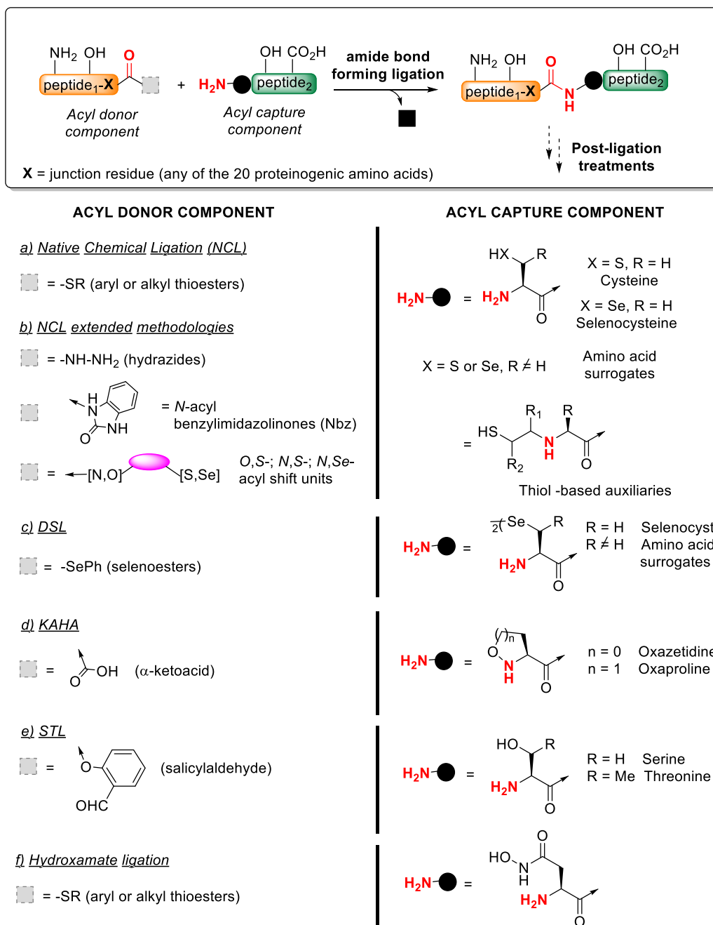
Figure 1. General principle of most commonly used chemoselective amide-bond forming reactions.
