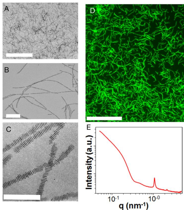
Figure 2: (A) and (B): lower and higher magnification TEM images of threads of 4 ML square platelets. (C) High-resolution TEM image of the threads showing the face to face stacking of CdSe platelets. (D) Fluorescence microscopy images of the threads deposited from solution on a cover slip. (E) Small angle X-ray scattering curve of the thread dispersion. Scale bars: 5 \mu\text{m} (A), 200 nm (B), 20 nm (C), 20 \mu\text{m} (D).
