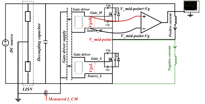
Fig. 2. Synchronous converter, double pulse test schematic.
