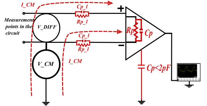
Fig. 4. Conventional differential probe
