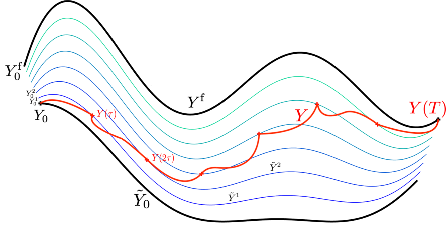
FIGURE 2. Schematic representation of the staircase method used for the proof of Theorem 2.8.
