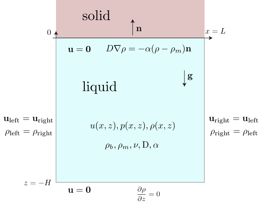
FIG. 2. (color online) Representation of the numerical domain with the appropriate boundary conditions.
