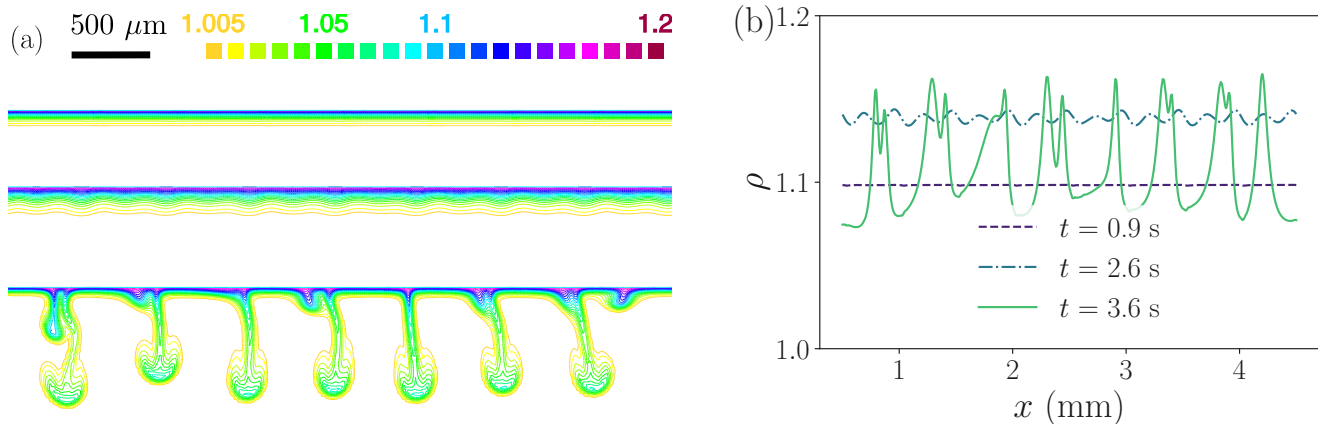
FIG. 3. (color online) (a) Snapshots of the simulation (case of the salt) at different times corresponding to the three regimes discussed in the main text: t = 0.9 s (diffusive regime); t = 2.6 s (instability regime); t = 3.6 s (plume regime). Each color represents an iso dimensionless density (see colorscale). (b) Quantitative density profiles at corresponding times. The graph represents the dimensionless density \rho(x) for a fixed distance from the interface ( z = -20 \mu\text{m} ).
