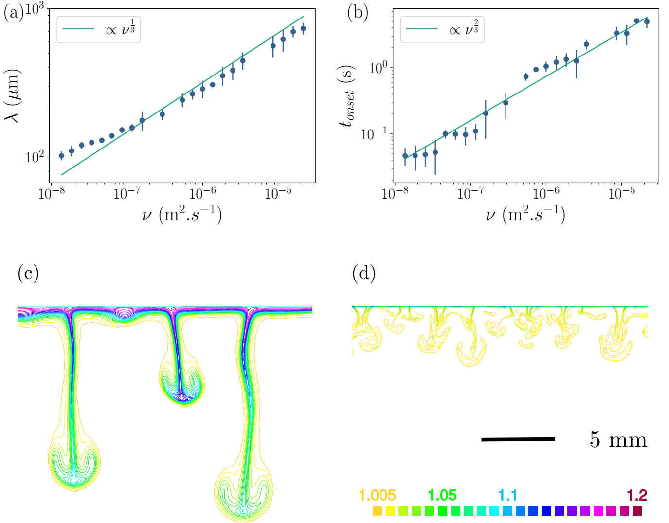
FIG. 7. (color online) Influence of the kinematic viscosity \nu . Wavelength \lambda (a) and onset time t_{onset} (b) as a function of the kinematic viscosity \nu . Data are well fitted with the scalings for fast dissolution kinetics Da \gg 1 of Eq. (7) and (8) respectively. Snapshots of plumes shortly after t_{onset} : (c) \nu = 10^{-5} \text{m}^2 \cdot \text{s}^{-1} and t \approx 2 t_{onset} ; (d) \nu = 10^{-7} \text{m}^2 \cdot \text{s}^{-1} and t \approx 5 t_{onset} . For both cases, scale is the same indicated by the 5mm scalebar. Isovalues for \frac{\rho}{\rho_b} are indicated by the color code.
