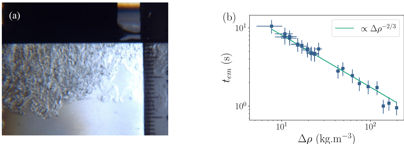
FIG. 1. (color online) (a) Shadowgraph image of solutal convective flow. A salt block is put in contact with fresh water and the image is taken 1.25 s after the contact. A graduation corresponds to 1 mm. (b) Emission time t_{em} of the first plume as a function of the density difference \Delta\rho = (\rho_m - \rho_b) , by adjusting the maximal density to \rho_m = 1195 \text{ kg.m}^{-3} . The straight line indicates the scaling t_{em} = K \left( \eta / (\Delta\rho g \sqrt{D}) \right)^{2/3} with the fitted value K = 12.8 .
