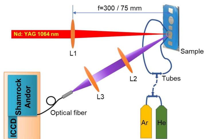
Figure 4 Experimental setup. L1-3: Fused silica plano-convex lens.
