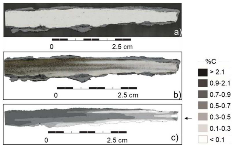
Figure 3 The optical microscopic images before (a) and after (b) Nital etching of the cross section of the archaeological sample; c) the obtained carbon content distribution.
