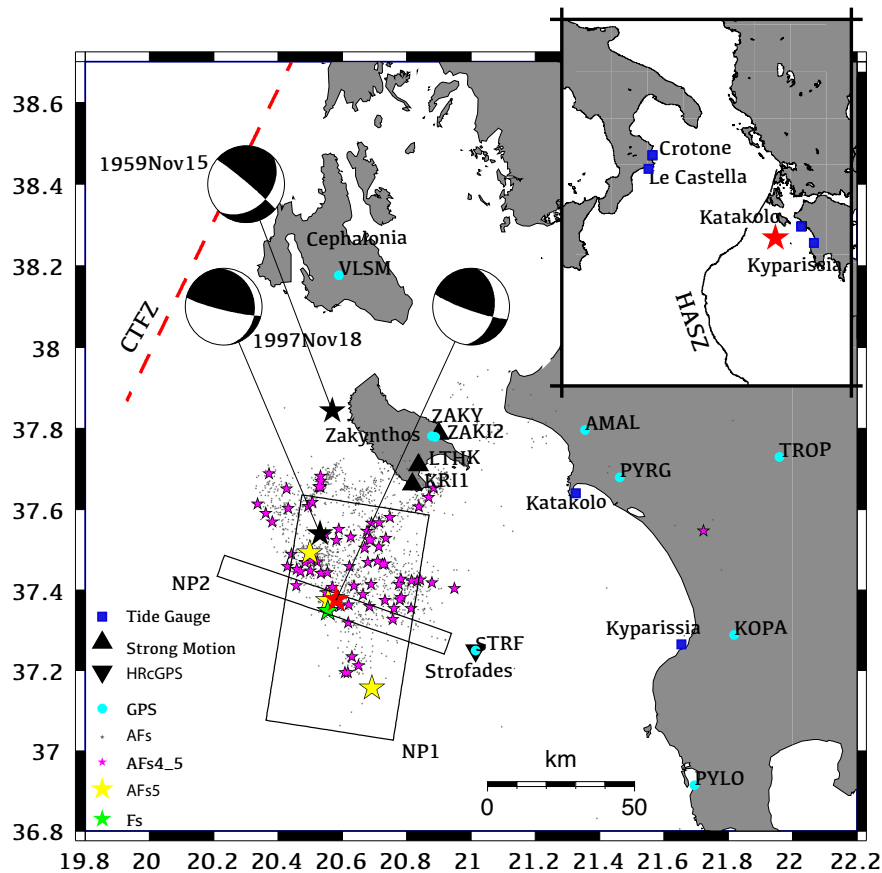
Figure 1. Location map of the 2018 Zakythos earthquake. Black triangles and inverted triangles represent the strong motions and the HRGPS stations, respectively. Cyan circles and blue squares (in the inset) represent the GPS sites and the tide gauges, respectively. The red star indicates the epicentre. Black boxes represent the surface projection of the fault planes corresponding to the NP1 and NP2 USGS focal mechanism solutions. Grey, pink, yellow and green stars, display all the aftershocks, those with magnitudes between 4 and 5, those with magnitude greater than 5 and the foreshock, respectively. Events with M > 4 have been relocated in this study (Table 2). Focal mechanisms of the 1959 and 1997 earthquakes are also displayed. Red dashed line shows the approximate position of the east-dipping Cephalonia Transform fault zone (CTFZ); black line in the inset displays the Hellenic Arc subduction zone [HASZ, Kreemer & Chamot-Rooke (2004)].
