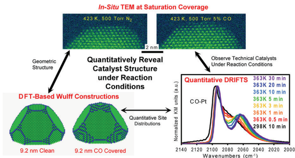
Figure 5. Illustration of the facet-selective surface reconstruction of carbon-supported Pt nanoparticles under CO pressure. Reprinted with permission from Ref. [67]. Copyright 2017 American Chemical Society.
