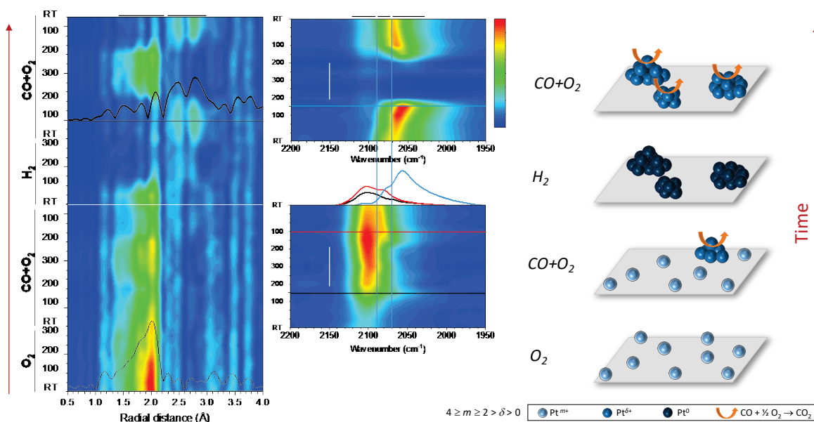
Figure 11. Operando EXAFS and DRIFTS monitoring of 0.3 wt% Pt/ \gamma -Al 2 O 3 catalyst in CO oxidation conditions (CO:O 2 =2:10%), after calcination or reduction. Y-scales indicate temperatures in °C. Color Z-scales represent EXAFS FT module and IR absorbance. The picture at the right-hand side illustrates the state of the Pt species at each step. Adapted from Ref. [10].
