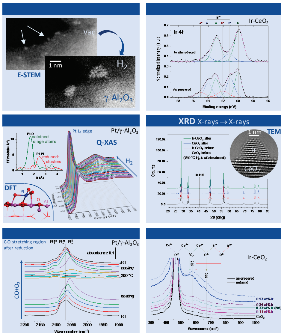
Figure 4. Examples of in situ characterization of supported nanocatalysts and single-atom catalysts. The left-hand-side panel corresponds to Pt/Al 2 O 3 SACs (adapted from Refs. [10,20]), while the right-hand-side panel relates to Ir/CeO 2 catalysts synthesized by one-step solution combustion (adapted from Ref. [21]). Incoming and outgoing radiation types are indicated. Acronyms are explained in Table 1.
