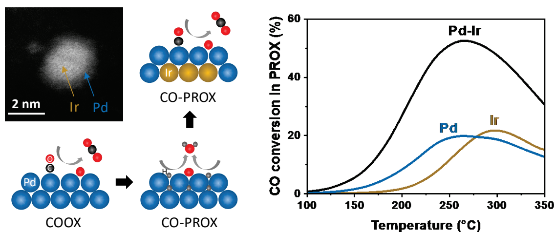
Figure 7. Illustration of Pd hydriding and alloying effects on CO oxidation during PROX. The STEM-ADF image shows an Ir@Pd core-shell nanoparticle supported on carbon. The graph plots CO conversion vs temperature during CO-PROX reaction ( CO:O_2:H_2:He = 2:2:48:48\% ) over Pd, Ir, and Pd-Ir NPs supported on amorphous silica-alumina (adapted from Ref. [165]).
