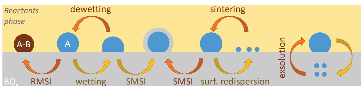
Figure 12. Illustration of reaction medium/metal particle/oxide support interaction phenomena in heterogeneous catalysis. Large disks represent nanoparticles or clusters, while small ones represent single atoms. Orange and yellow arrows denote (most frequently) reductive and oxidative processes, respectively. SMSI and RMSI stand for strong metal-support interaction and reactive metal-support interaction, respectively.
