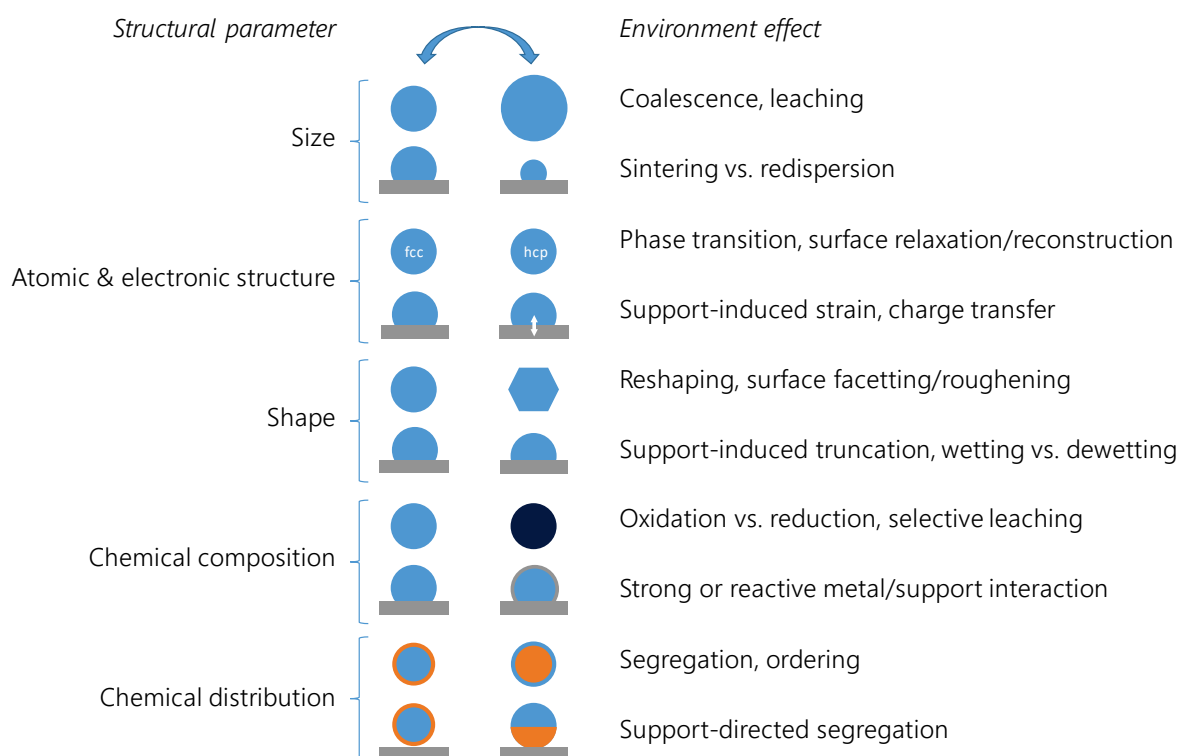
Figure 2. Examples of NP structural changes induced by the catalytic environment.
