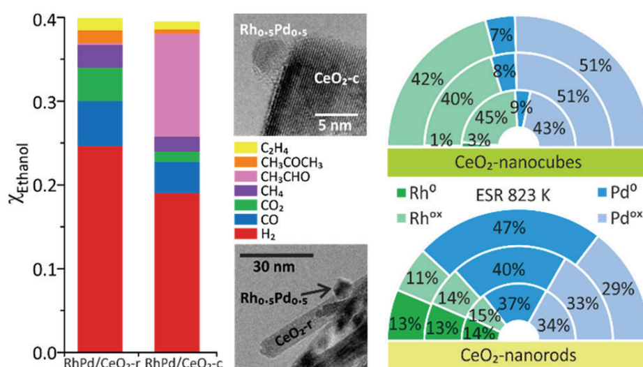
Figure 8. Illustration of the differences in catalytic selectivities (left) and depth-dependent compositions (right) between Rh-Pd NPs supported on ceria nanocubes and ceria nanorods under ethanol steam reforming conditions. TEM images of the two catalysts are displayed. Reprinted with permission from Ref [198]. Copyright 2019 American Chemical Society.
