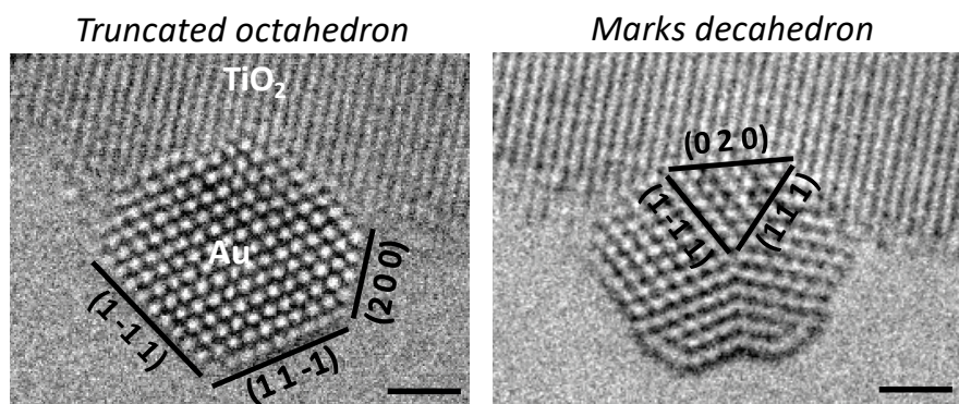
Figure 6. Aberration-corrected ETEM images (FEI Titan ETEM G2 300 kV) showing the (reversible) shape change, from octahedron to decahedron, of a gold nanoparticle supported on rutile TiO_2 at 300 °C under 0.5 mbar O_2 .
