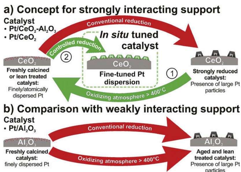
Figure 10. a) Dynamic nature of Pt on ceria is exploited to adjust noble metal dispersion. 1) The noble metal is finely dispersed on CeO 2 during oxidative treatment by exploiting metal–support interaction with ceria. 2) Formation of slightly larger noble metal particles is initiated by the application of controlled reducing steps (for example, pulses) at a low temperature (<400 °C). b) Redispersion step is not applicable at moderate temperatures for weakly interacting supports like Al 2 O 3 . Reprinted with permission from Ref. [234]. Copyright 2017 Wiley.
