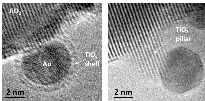
Figure 9. Aberration-corrected ETEM images (FEI Titan ETEM G2 300 kV), recorded under 0.5 mbar of atmospheric air at 300 °C, showing a rutile \text{TiO}_2 -supported Au NP encapsulated in a Ti oxide shell (left), and the same NP extracted from the shell with the formation of a rutile \text{TiO}_2 “nanopillar” (right). The extracted state was generated by condensing the TEM electron beam.
