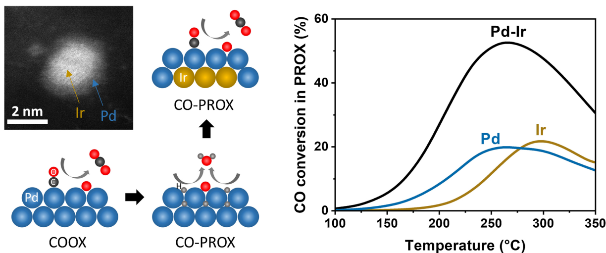
Fig. 7. Illustration of Pd hydriding and alloying effects on CO oxidation during PROX. The STEM-ADF image shows an Ir@Pd core-shell nanoparticle supported on carbon. The graph plots CO conversion vs temperature during CO-PROX reaction (CO:O 2 :H 2 :He = 2:2:48:48 %) over Pd, Ir, and Pd-Ir NPs supported on amorphous silica-alumina.
