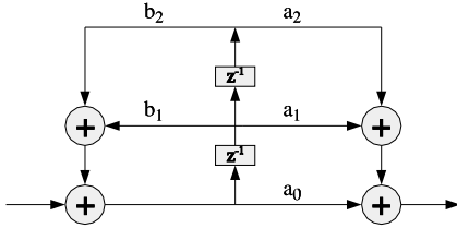
Figure 4: Filter: direct form II ( 2 zeros, 2 poles)
