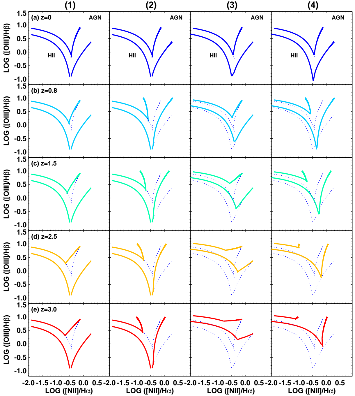
Figure 5. The Cosmic BPT Diagram: Our theoretical predictions for the position of the star-forming abundance sequence (left curve) and the starburst-AGN mixing sequence (right curve). The primary driver for our BPT evolution model is chemical enrichment. The rows give the expected position of the two sequences as a function of redshift for four limiting model scenarios given in each column. Column (1): Normal ISM conditions, and metal-rich AGN NLR at high- z ; Column (2): Normal ISM conditions, and metal-poor AGN NLR at high- z ; Column (3): Extreme ISM conditions, and metal-rich AGN NLR at high- z ; Column (4): Extreme ISM conditions, and metal-poor AGN NLR at high- z .
