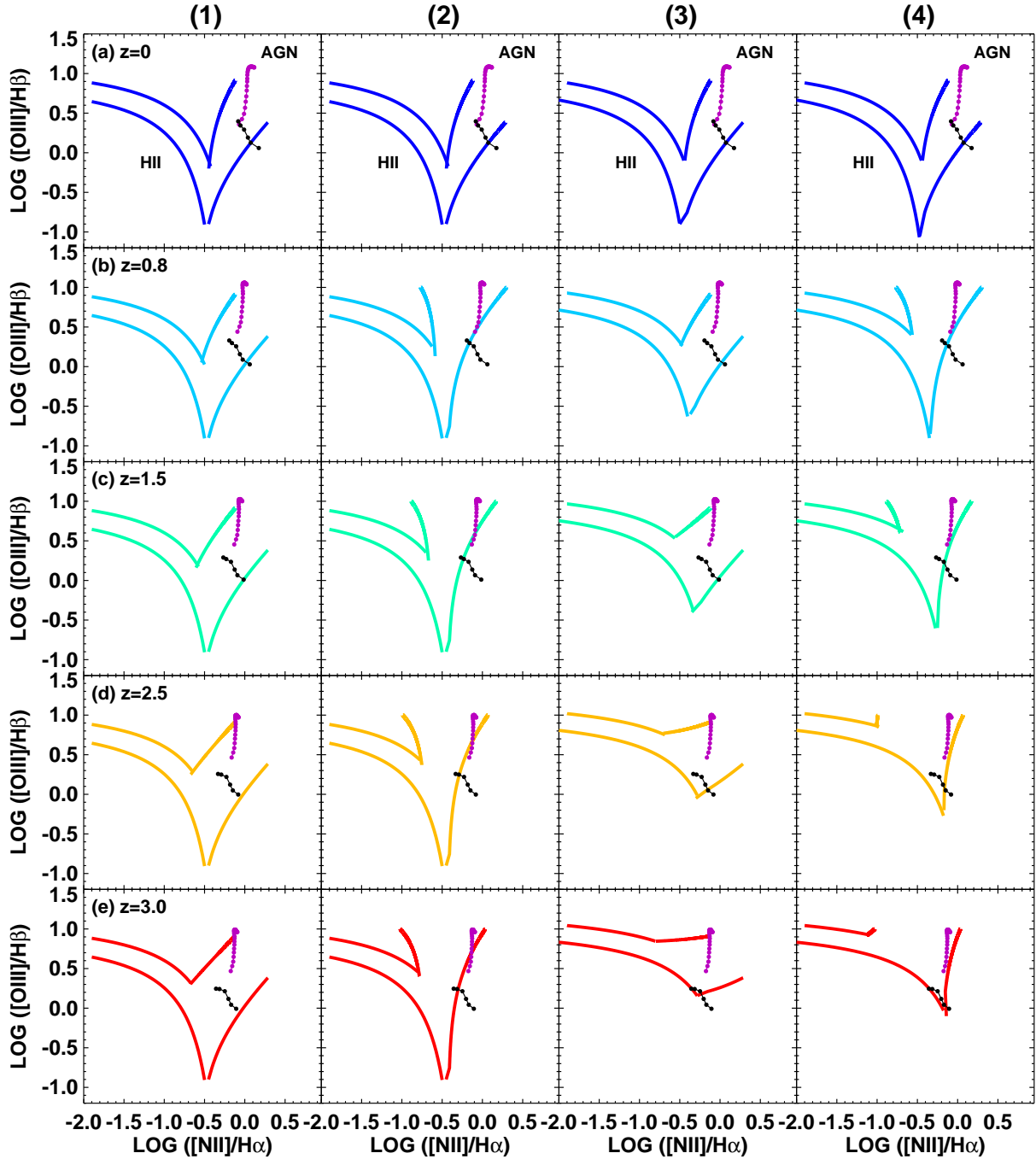
Figure 7. The Cosmic BPT Diagram: Our theoretical predictions for the position of the star-forming abundance sequence (left curve) and the starburst-AGN mixing sequence (right curve) as a function of redshift (rows) for our four limiting scenarios (columns) described in Section 5. In our model, the primary drivers for BPT evolution are chemical enrichment and a change in the ISM conditions for star-forming galaxies. The (Allen et al. 2008) fast shock models (purple) and the (Rich et al. 2010) slow shock models (black) are shown for comparison.
