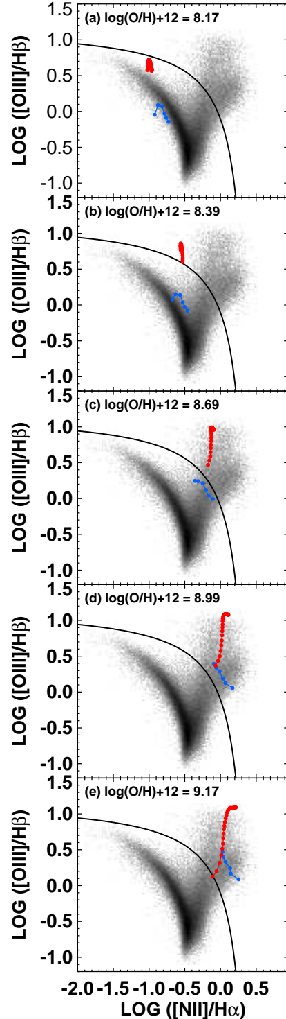
Figure 6. The (Allen et al. 2008) fast shock models (red) and the (Rich et al. 2010) slow shock models (blue) as a function of metallicity. For comparison, the SDSS sample from (Kewley et al. 2006b) is shown. The fast and shock slow model positions indicate where galaxies that are 100% dominated by shocks are likely to lie. Galaxies containing a mixture of ionizing sources, such as shocks and star-formation will lie along mixing sequences between the star-forming sequence and the 100% shock models. The position and shape of the mixing sequences will depend on the metallicity of the galaxy and the shock velocity. Examples of typical mixing sequences are given in Rich et al. (2010, 2011).
