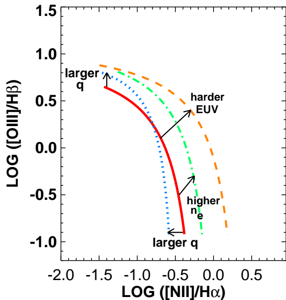
Figure 2. An illustration of the effect of varying different galaxy parameters on the star-forming galaxy abundance sequence in the [N II]/H \alpha versus [O III]/H \beta diagnostic diagram. The original SDSS star-forming galaxy sequence is well-fit by the red theoretical curve. Raising the hardness of the ionizing radiation field (orange dashed line) moves the abundance sequence towards larger [N II]/H \alpha and [O III]/H \beta ratios. A similar effect is seen when the electron density of the gas is raised (green dot-dashed line). The relationship between ionization parameter, metallicity and the [N II]/H \alpha and [O III]/H \beta line ratios is more complex. At high metallicities, raising the ionization parameter causes the [N II]/H \alpha ratio to become smaller, while [O III]/H \beta is largely unaffected. At low metallicities, raising the ionization parameter raises the [O III]/H \beta ratio while [N II]/H \alpha is largely unaffected.
