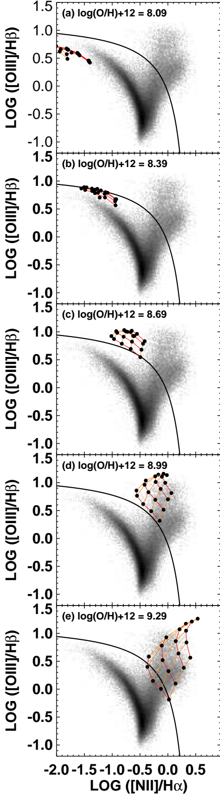
Figure 4. The (Groves et al. 2004a) dusty radiation pressure dominated photoionization models for AGN as a function of metallicity. Lines of constant ionization parameter (orange) and constant power-law index (red) are shown. For comparison, the SDSS sample from (Kewley et al. 2006b) is shown.
