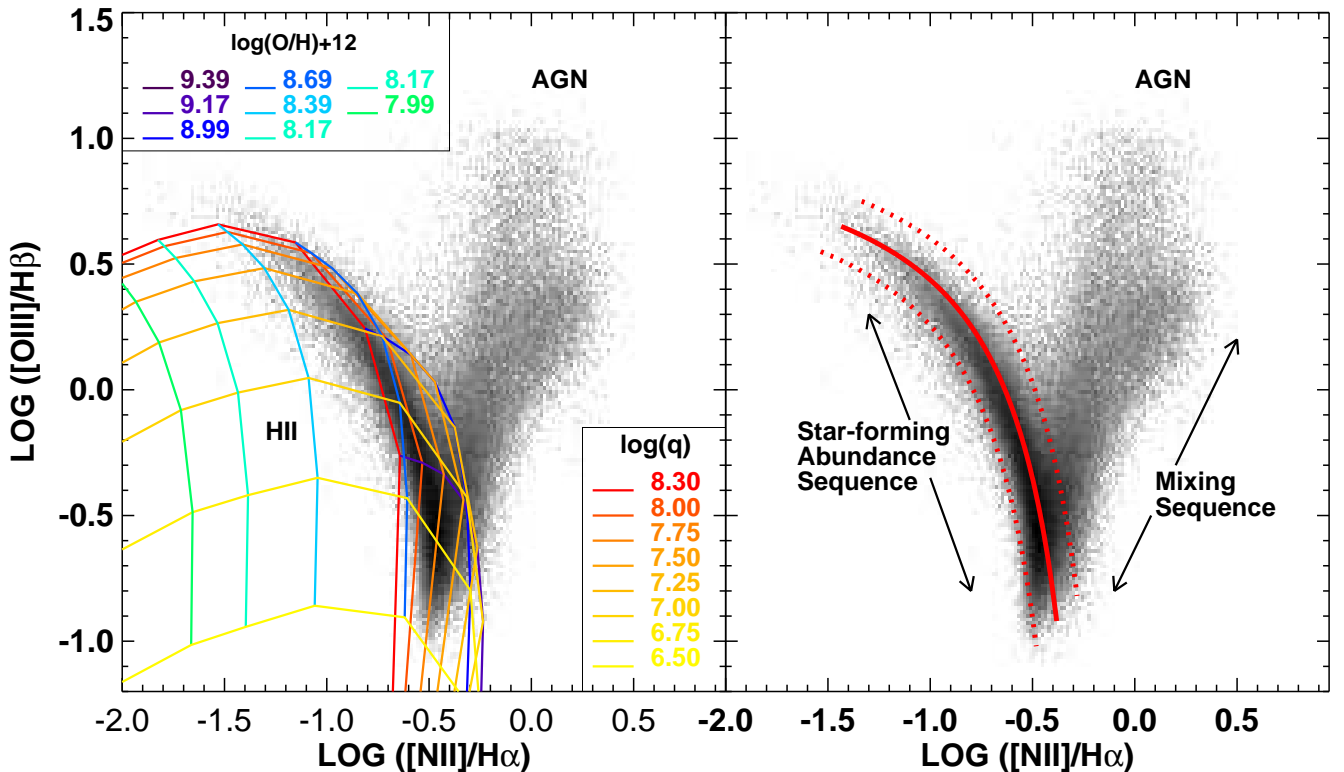
Figure 1. The [\text{N II}]/\text{H}\alpha versus [\text{O III}]/\text{H}\beta optical diagnostic diagram for the Sloan Digital Sky Survey galaxies analyzed by Kewley et al. (2006b). Left: The colored curves show our new theoretical stellar population synthesis and photoionization model grid for star-forming galaxies based on a \kappa electron temperature distribution. Right: The red solid curve shows the mean star-forming sequence for local galaxies. The shape of the red solid curve is defined by our theoretical photoionization models, while the position is defined by the best-fit to the SDSS galaxies. The \pm 0.1 dex curves (dashed lines) represent our model errors and contain 91% of the SDSS star-forming galaxies.
