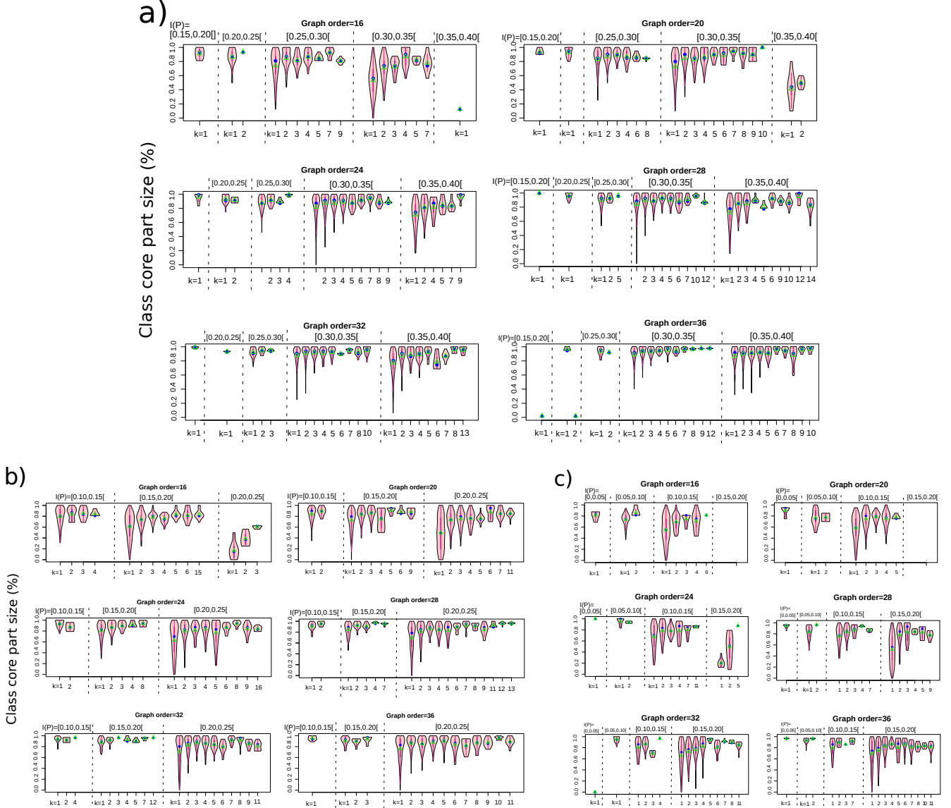
Figure 9: Proportion of the graph covered by the class core parts, as a function of the detected imbalance I(P) and number of classes k , (a) for l_0 = 2 , (b) for l_0 = 3 and (c) for l_0 = 4 . Notice that an x -axis value may be empty if the parameter set is not defined or no data is available. Plots available at 10.6084/m9.figshare.8233340 under CC-BY license.
