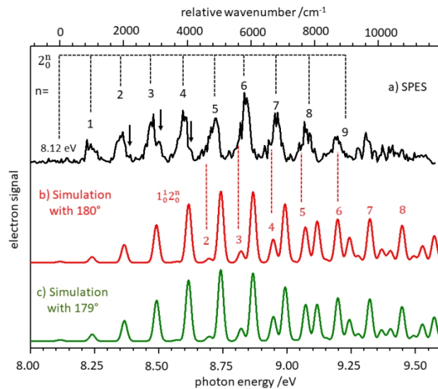
Fig. 2 SPES of 11BH 2 along with the spectral simulations. Simulated spectra are shifted by \sim 0.09 eV to lower energy to attend the best match with the experimental one. The origin transition, corresponding to the IE is determined as 8.12 eV. The first band in the SPES is assigned as 2_0^1 transition by comparing the band intensities between experiment and simulation.
