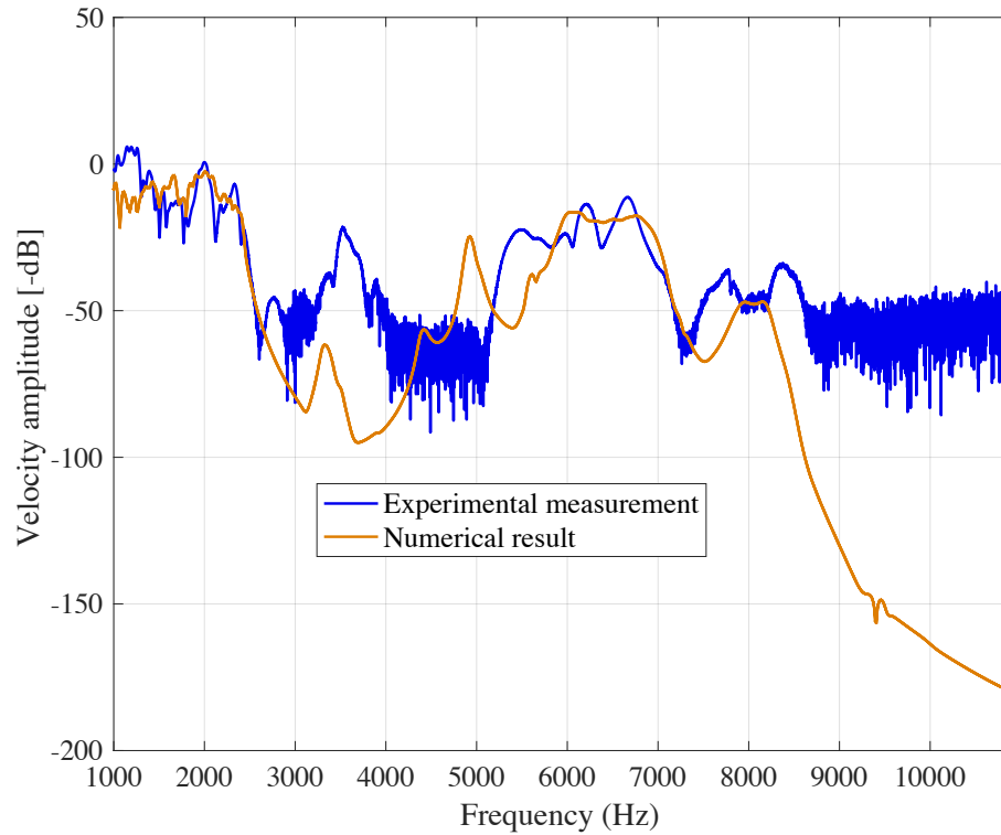
Figure 22: Comparison of numerical and experimental FRFs
