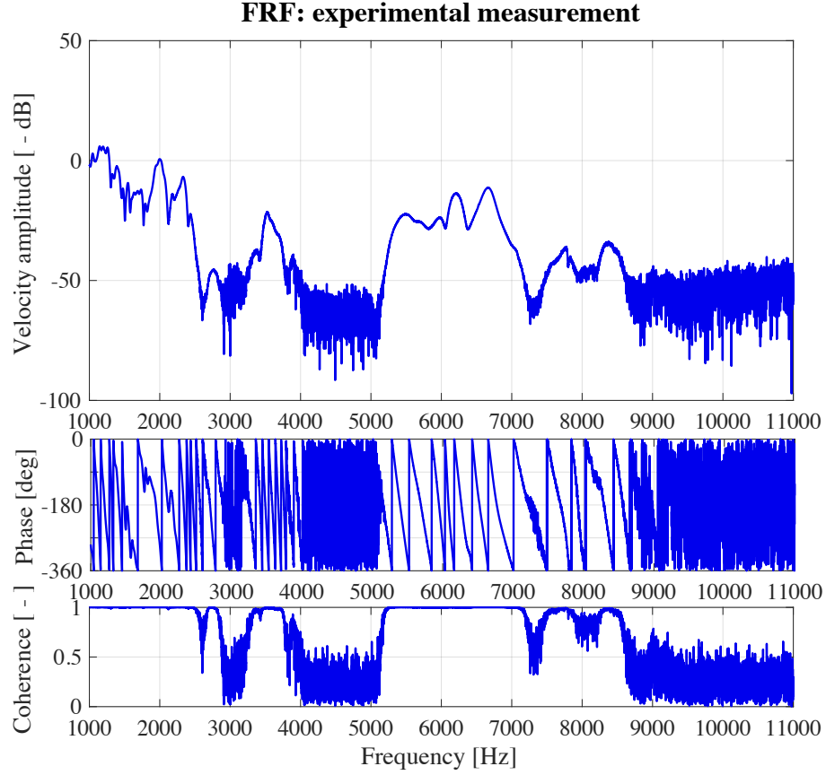
Figure 14: Velocity response measured in the output point
