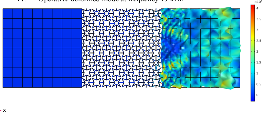
IV. Operative deformed mode at frequency 19 kHz
