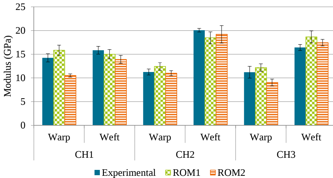
Figure 15: Comparison of experimental modulus and predicted modulus of composites
