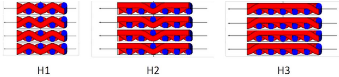
Figure 3: Schematic view of the stacking sequence in compaction tests (weft direction in red, warp direction in blue)
