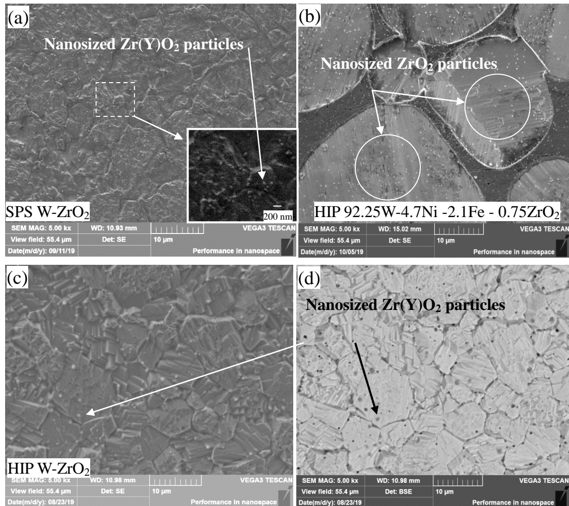
Fig. 16. Microstructure of alloys fabricated by different sintering process: (a) SPS process, (b) HIP sintering process, (c) HIP sintering process and (d) HIP sintering process (BSE image).
