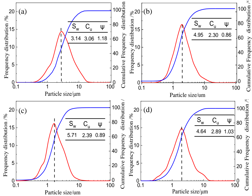
Fig. 11 PSDs of W- Zr(Y)O_2 powders with different Zr(Y)O_2 contents: (a) 0, (b) 0.25% Zr(Y)O_2 , (c) 0.5% Zr(Y)O_2 and (d) 0.75% Zr(Y)O_2 .
