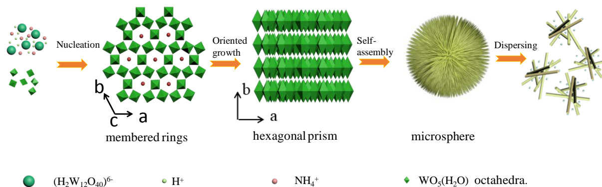
Fig. 3 Schematic diagram of morphology evolution mechanism of (\text{NH}_4)_{0.33}\text{WO}_3 \cdot \text{H}_2\text{O} precursor.
