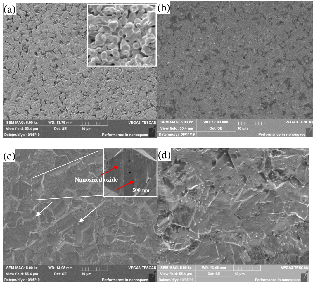
Fig. 13. Microstructure of alloys produced by different spark plasma sintering processes with various final temperatures: (a) 1800 °C for 5 min, (b) 1900 °C for 5 min, (c) 2000 °C for 5 min and (d) 2100 °C for 5 min.
