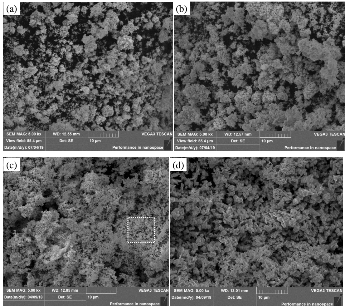
Fig. 6 Change of particle morphologies of doped powders obtained by different reduction processes at varying temperature: (a) 550 °C, (b) 650 °C, (c) 750 °C and (d) 800 °C, respectively.
