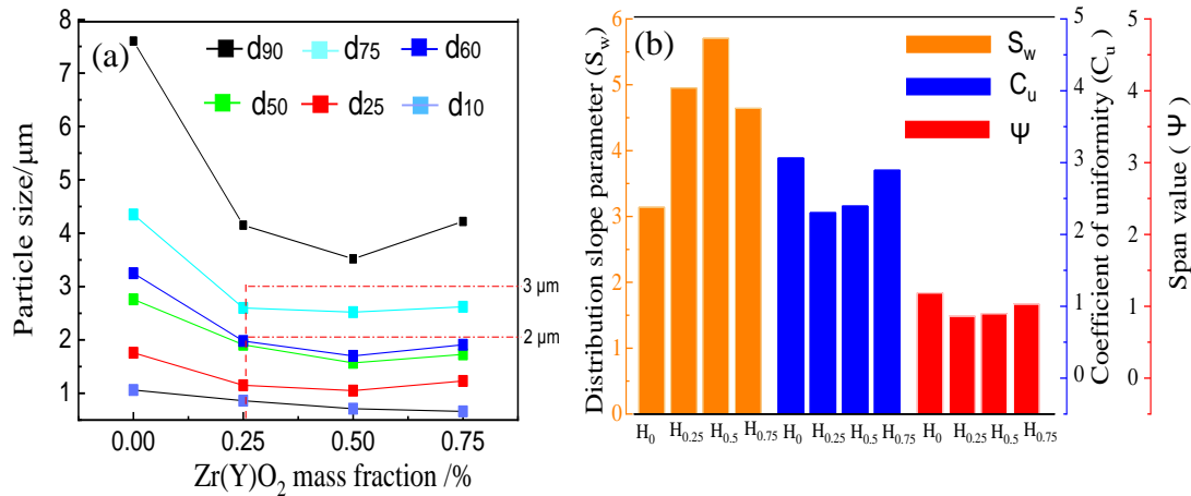
45 Fig. 12 PSD parameters of four W-Zr(Y)O 2 powders: (a) Particle sizes at the 46 different cumulative volume percentage vs. Zr(Y)O 2 content and (b) Distribution 47 slope parameter, coefficient of uniformity and span value vs. Zr(Y)O 2 contents. 48 49 50 51 52 53 54 55 56 57 58 59 60 61 62 63 64 65
