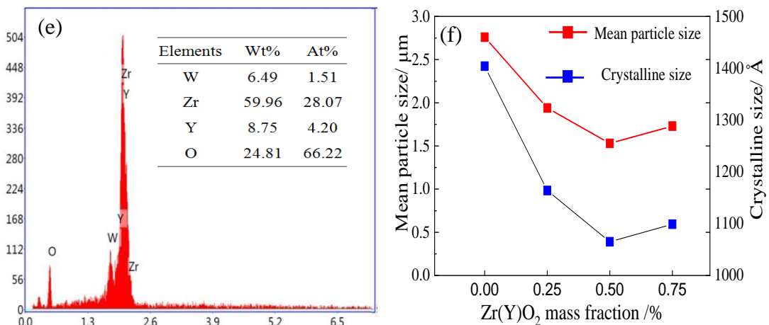
Fig. 8 Morphologies of doped tungsten powders: (a) Pure W, (b) W-0.25 wt% Zr(Y)O 2 , (c) W-0.5 wt% Zr(Y)O 2 , (d) W-0.75wt% Zr(Y)O 2 , (e) EDS pattern of the nanosized substance of red arrow A and (f) Mean particle size and crystalline size vs. Zr(Y)O 2 contents.
