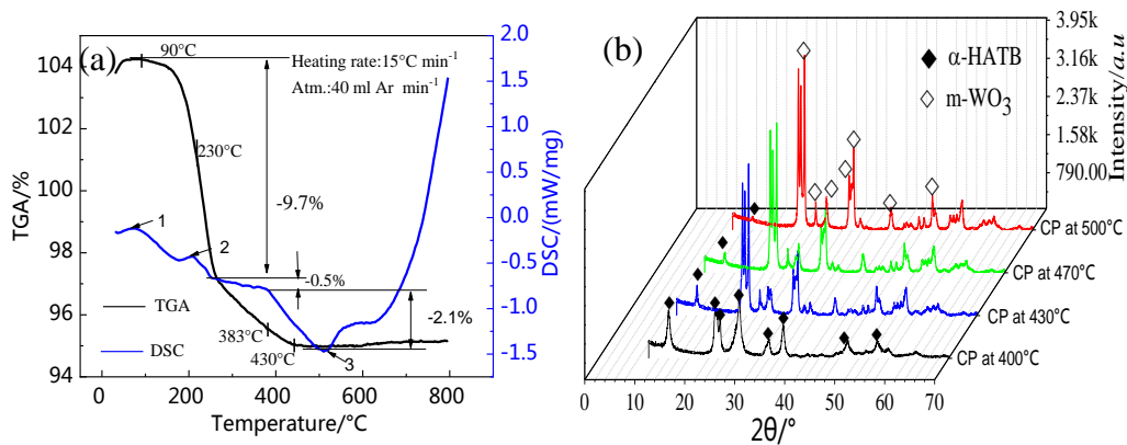
Fig. 4 (a) The TGA and DSC curves of the decomposition of the H_{0.5} precursor powder and (b) XRD patterns of doped powder after calcination at different temperature for 2 h.
