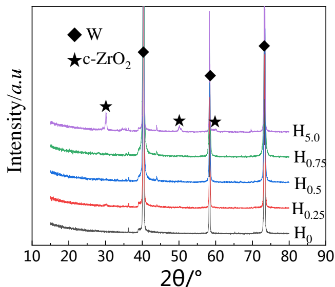
Fig. 7 XRD patterns of five doped powders after reduction at 900 °C for 2 h.
