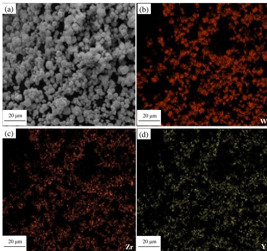
Fig. 9 Elemental distributions of the W-0.75wt% Zr(Y)O 2 powder.
