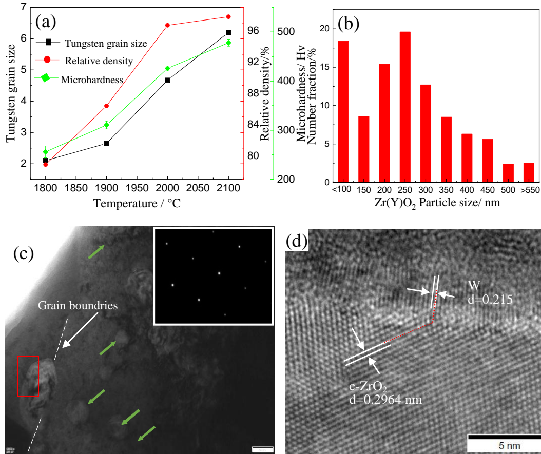
Fig. 14 (a) Evolution of tungsten grain, relative density and microhardness of alloy vs alloys sintered under different conditions, (b) PSD of Zr(Y)O 2 in alloy, (c) TEM images of tungsten alloy conducted of sintered alloy at 2000 °C and (d) HR-TEM image of Zr(Y)O 2 /W interface.
