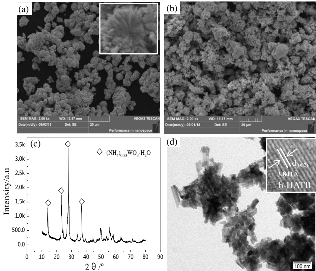
Fig. 2 (a) and (b) SEM images of the undoped and doped precursor powders, (c) XRD patterns of doped precursor powder and (d) TEM image of the H_{0.75} doped precursor.
