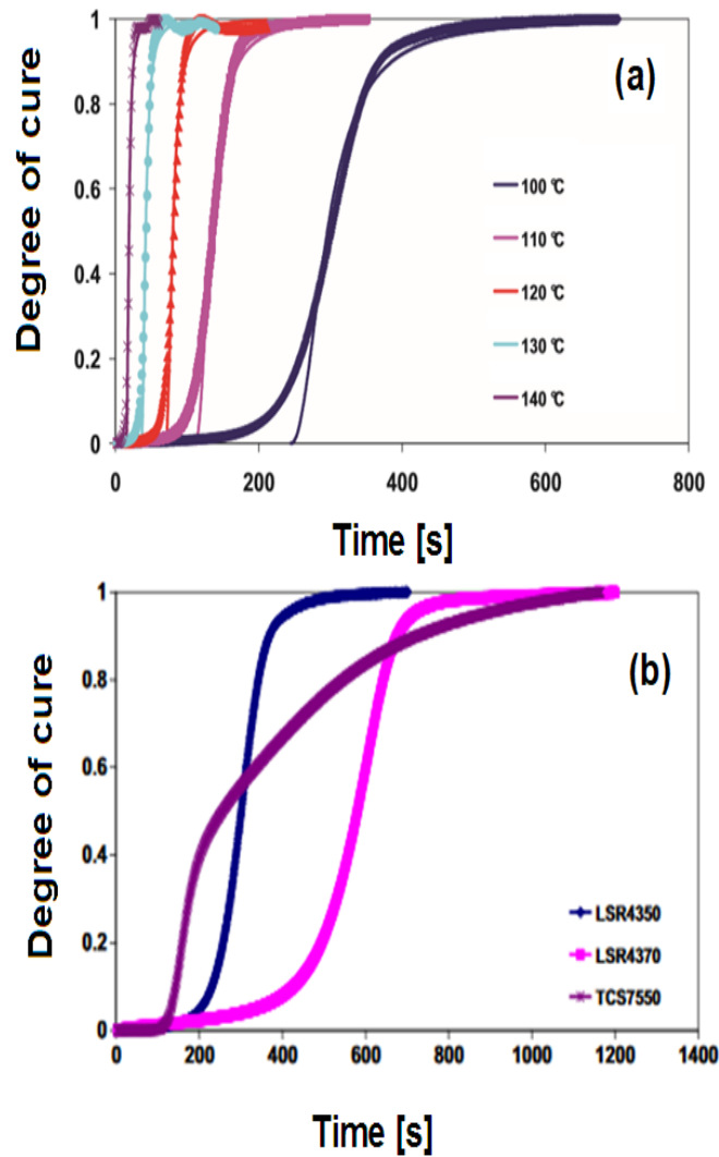
Figure 7. Experimental data of full cycles of curing versus time obtained at (a) various temperatures with LSR4350 and (b) 100 °C with the indicated liquid silicone rubber materials.
