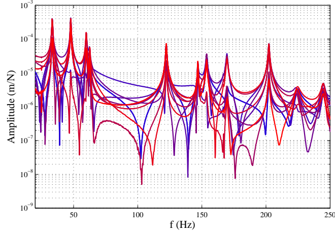
Fig. 8. Measured FRFs
