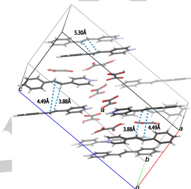
Figure 2. Packing arrangement of stilbazole A1 -oxalic acid 3:4 cocrystal CC1 obtained by cocondensation
