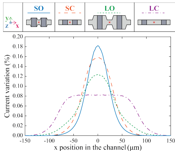
Fig. 14 Simulation of the current variation due to an 8 μm diameter polystyrene bead for conventional and optimised coplanar designs with an inter-electrode distance of 50 μm (SC and SO) and 150 μm (LC and LO). Adapted by permission from Cottet et al. 37 , Springer Nature, copyright 2019.
