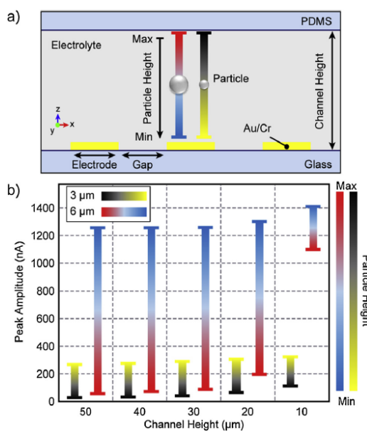
Fig. 15 Illustration of signal variations as a function of channel height. Red-blue gradient bar represents the height range of a 6 μm particle; black-yellow gradient bar represents the height range of a 3 μm particle. Electrode and gap widths are 10 μm. Adapted from Bilican et al. 43 with permission from Elsevier, copyright 2020.
